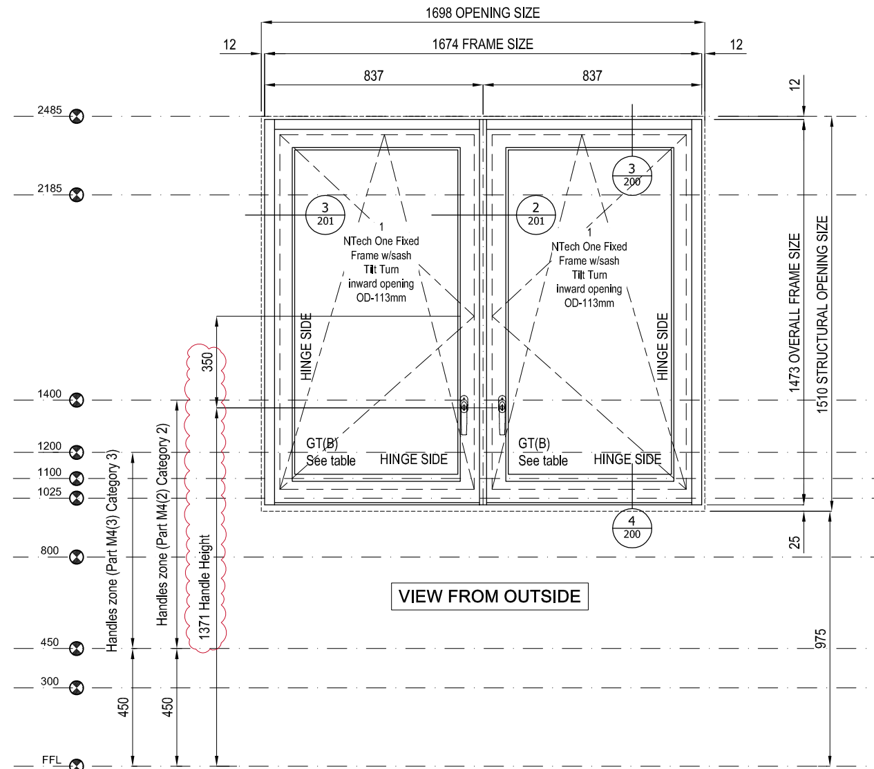
WINDOW TYPE WT-06
