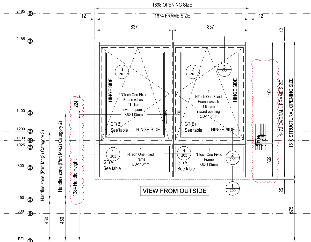
WINDOW TYPE WT-03A, WT-03B & WT-03C
