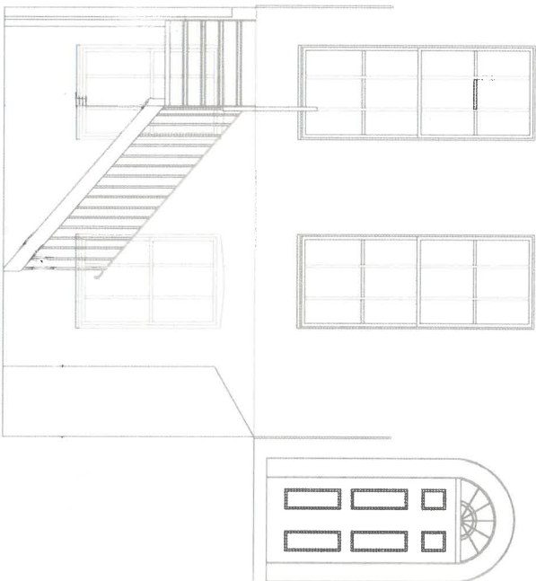
Existing West Elevation Lightwell
