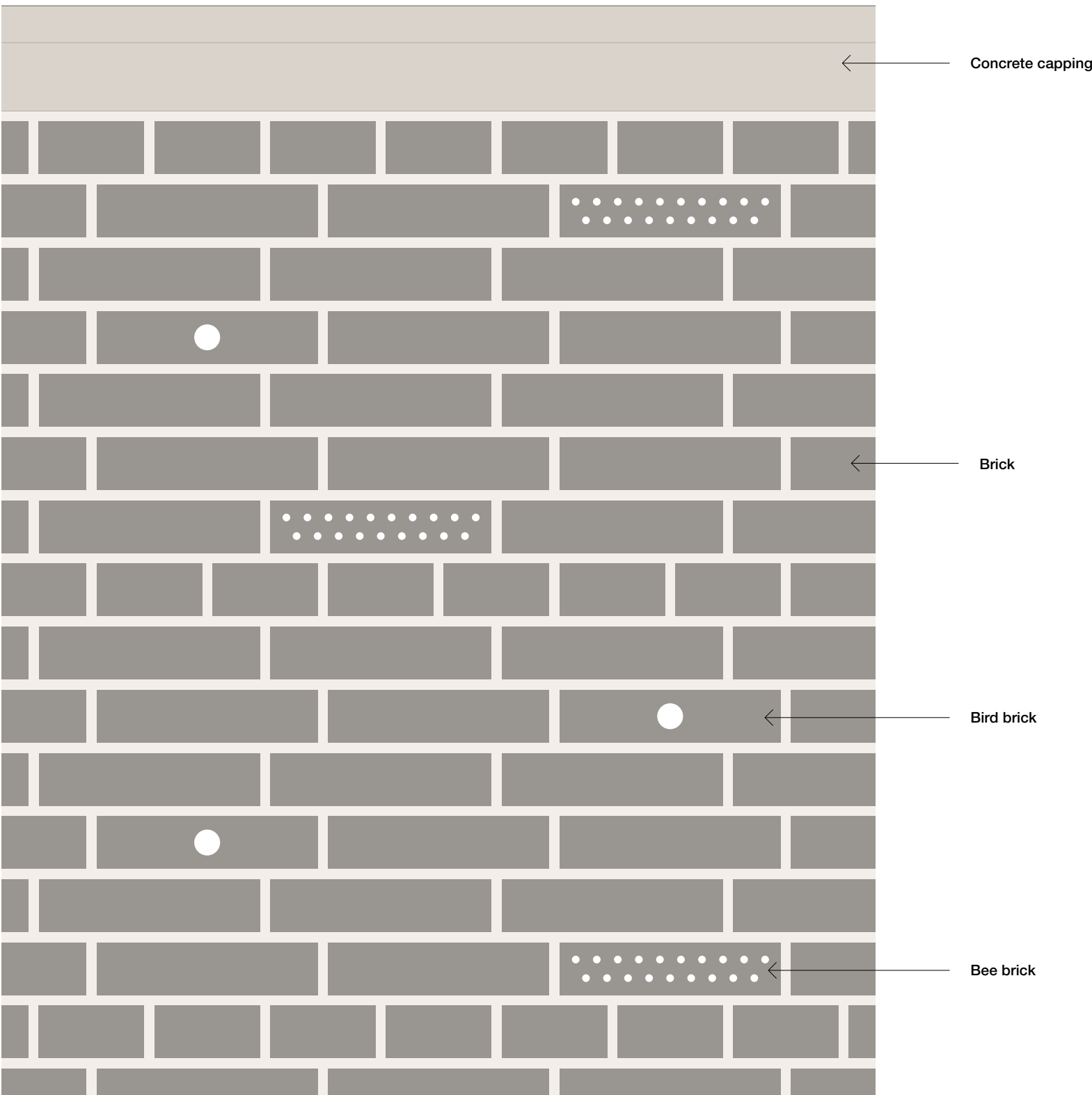
03 Indicative detail of brickwork with integrated habitats 1:10 @A3
