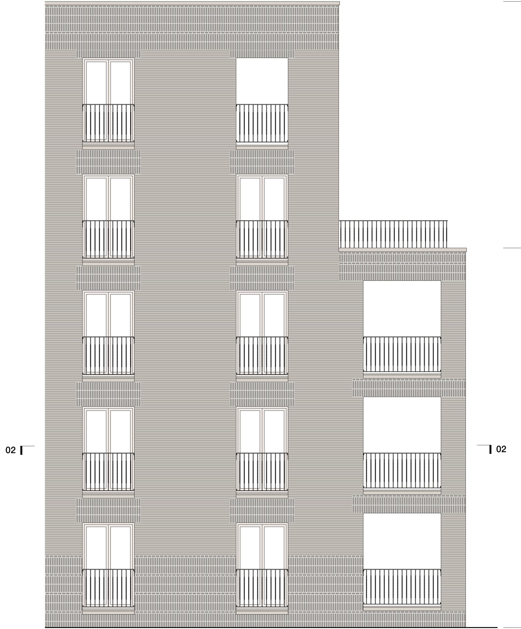
01 Elevation study An indicative bay of windows and loggias
