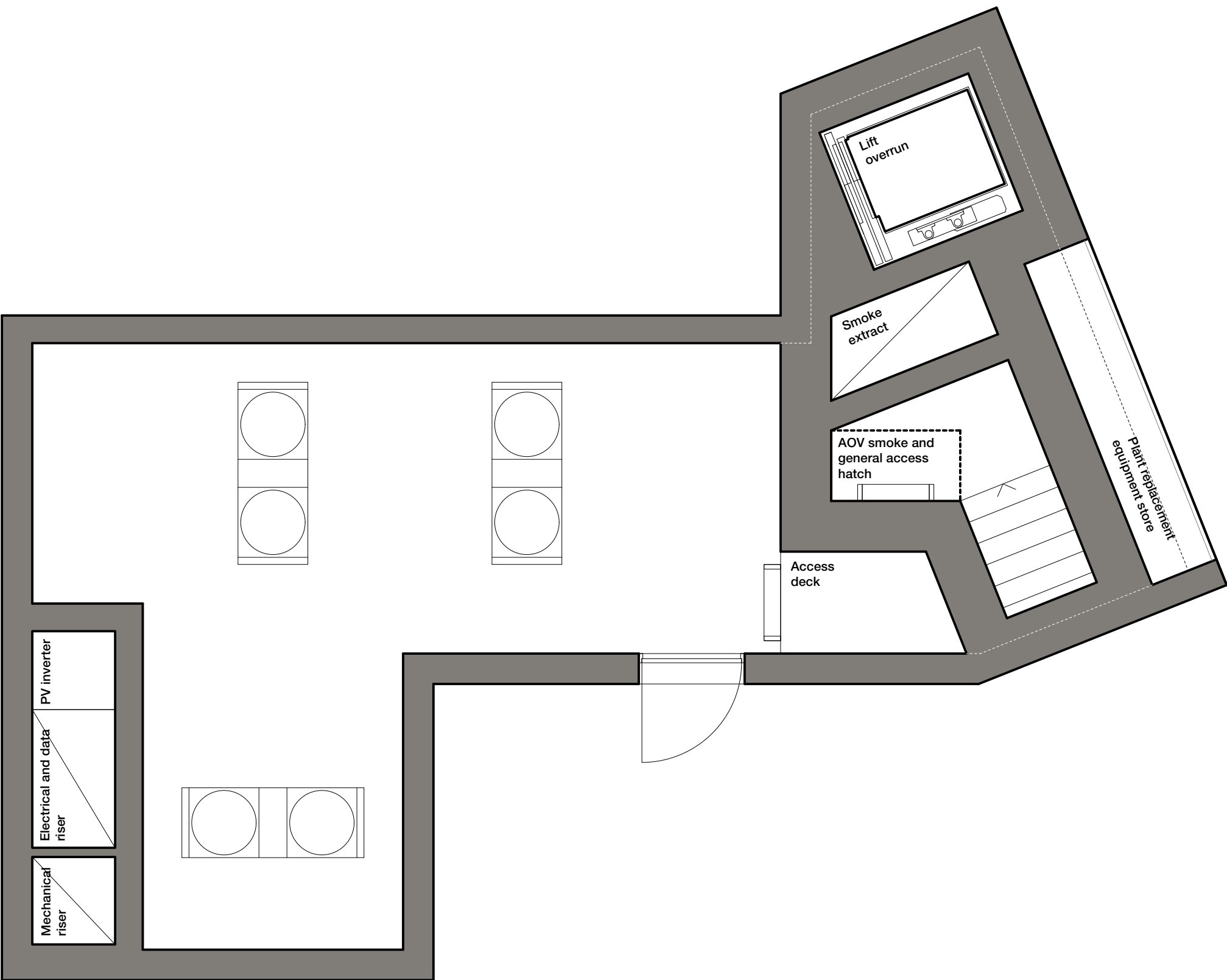
01 Plan of rooftop enclosure 1:100 @A3
