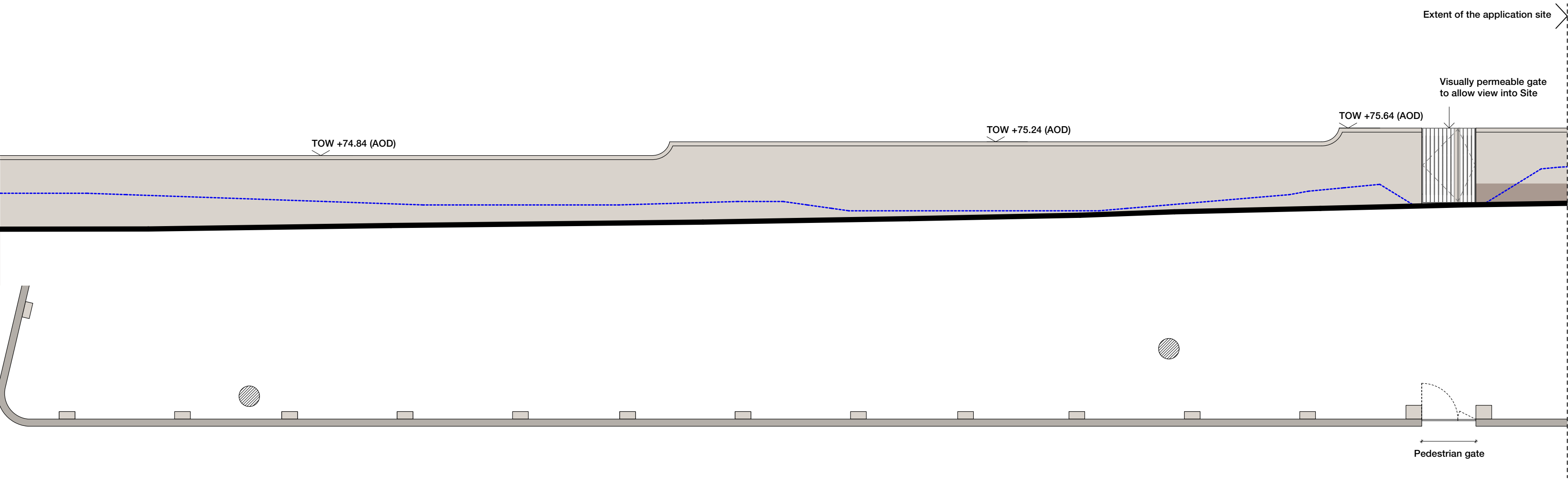
02 Nutley Terrace Boundary wall proposal
