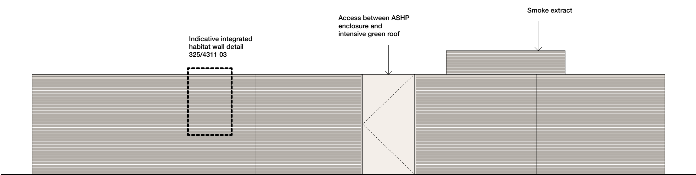
02 South elevation of rooftop enclosure 1:100 @A3
