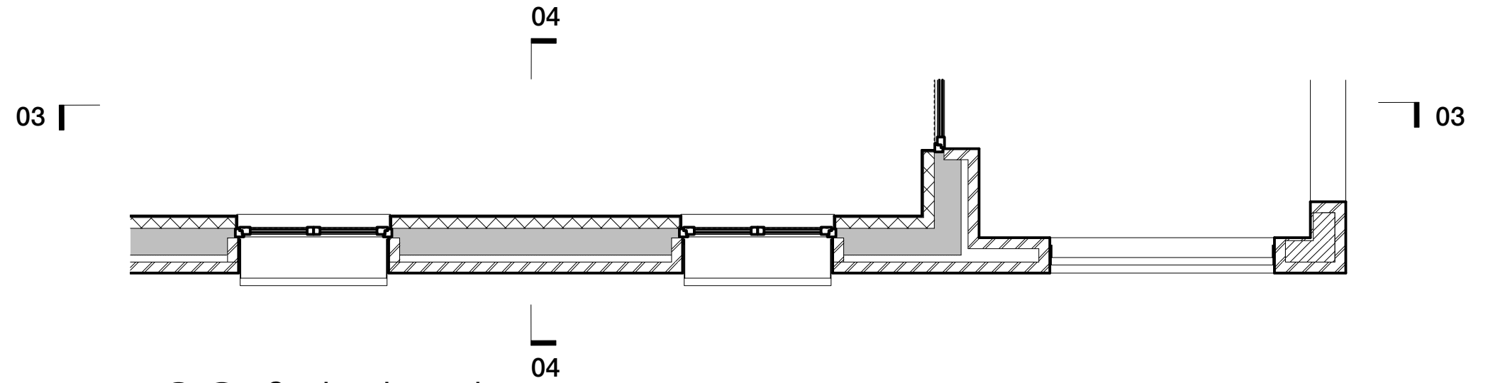
02 Section plan study Typical wall build-up and window openings
