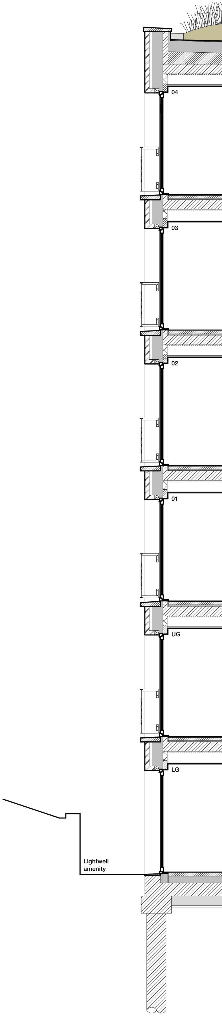
04 Section study Typical envelope and LGF lightwell
