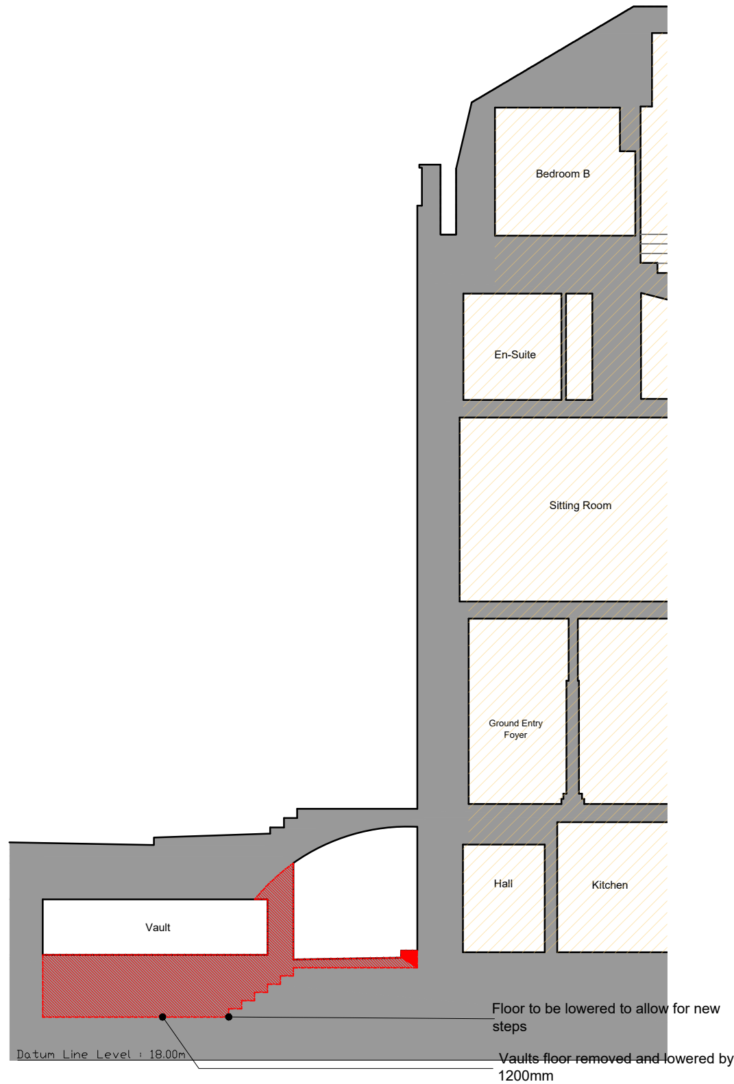
2 Demolition Section B-B GHV 1:100 @ A3
