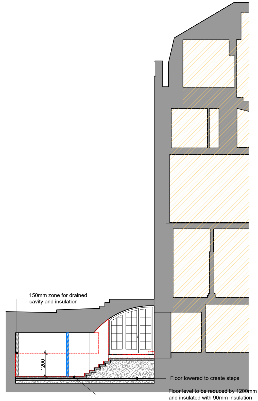
3 Proposed Section B-B GHV 1:100 @ A3
