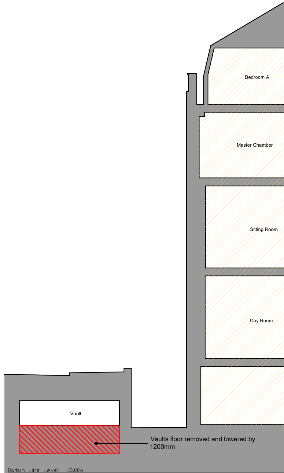
2 Demolition Section A-A GHV 1:100 @ A3
