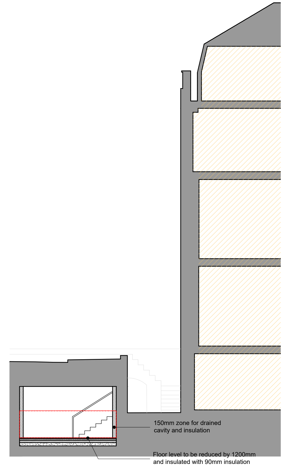
3 Proposed Section A-A GHV 1:100 @ A3
