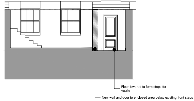
2 Proposed Elevation 02 GHV 1:100 @ A3
