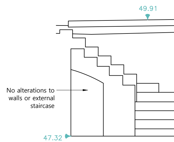
4 - Side Elevation
