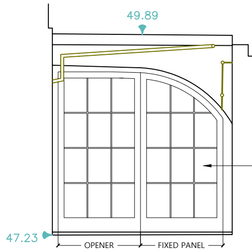
2 - Side Elevation
