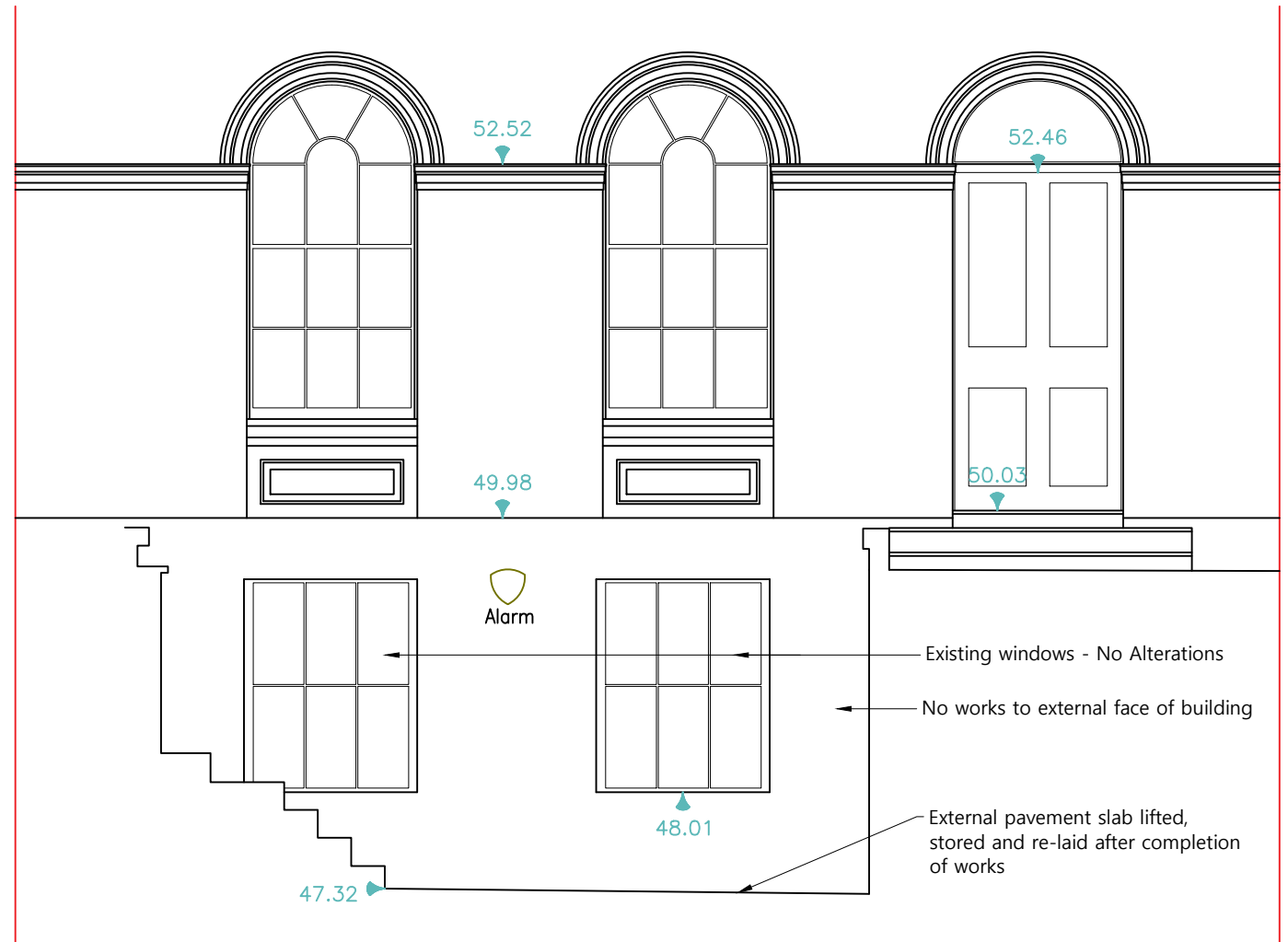
1 - Front Elevation
