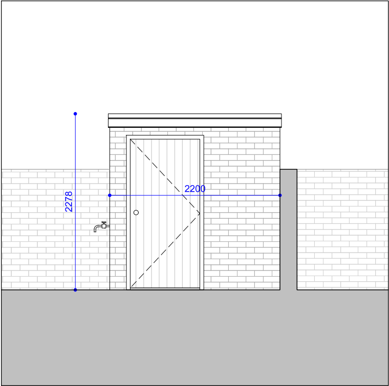
01. Garden Store Front Elevation
