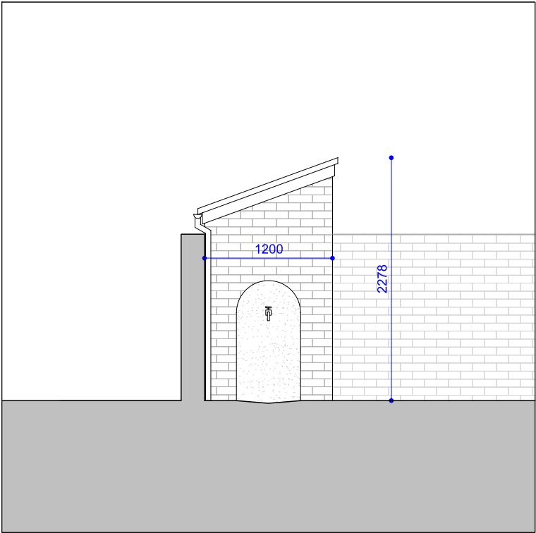
02. Garden Store Side Elevation
