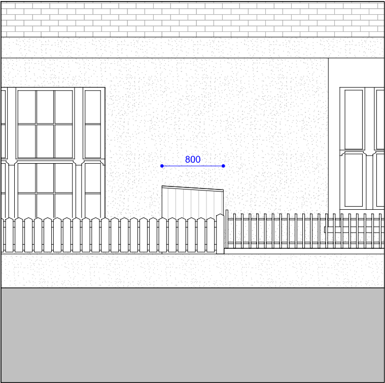
04. Bin Store Side (street) Elevation
