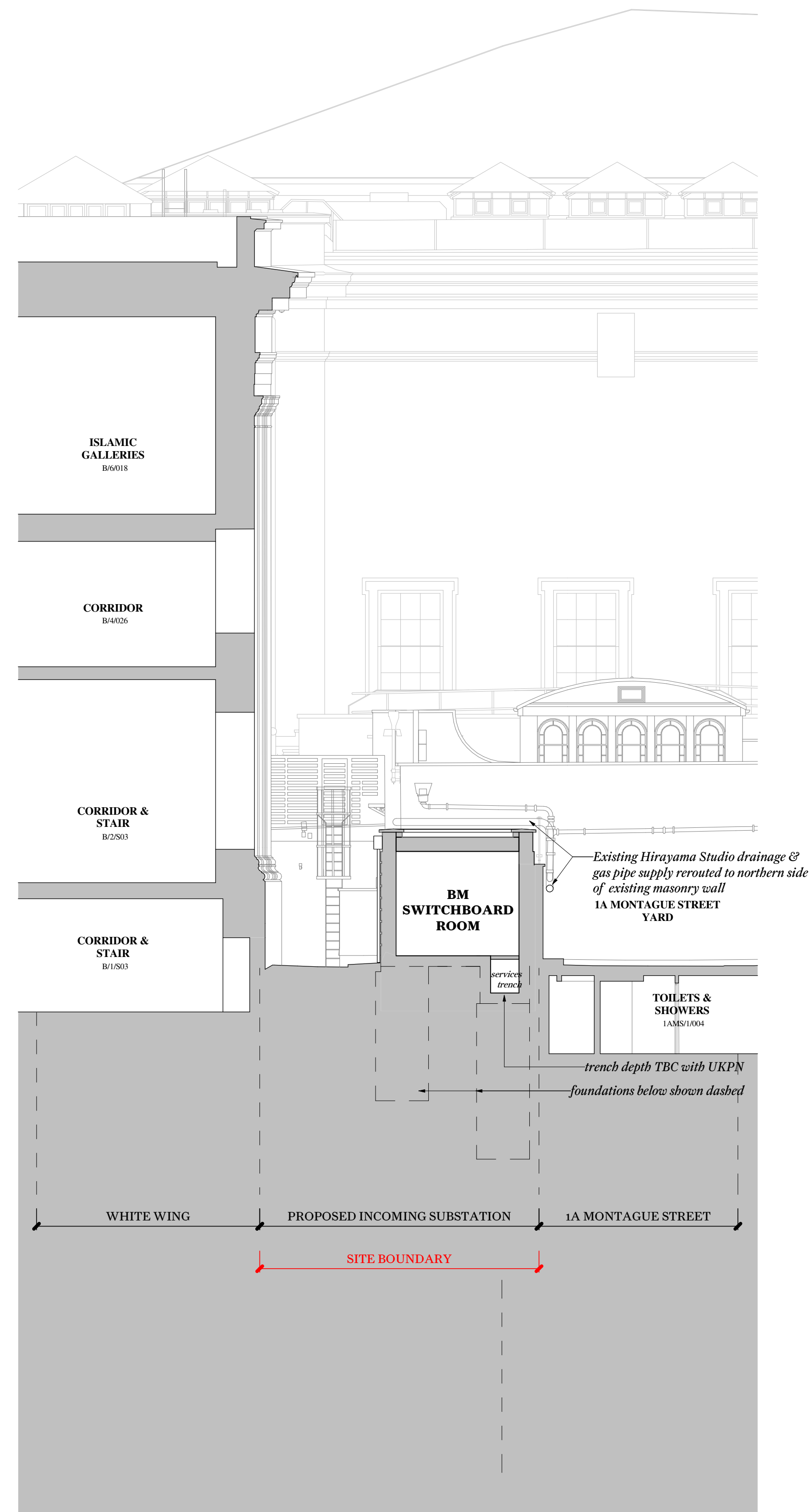
Proposed Section CC
