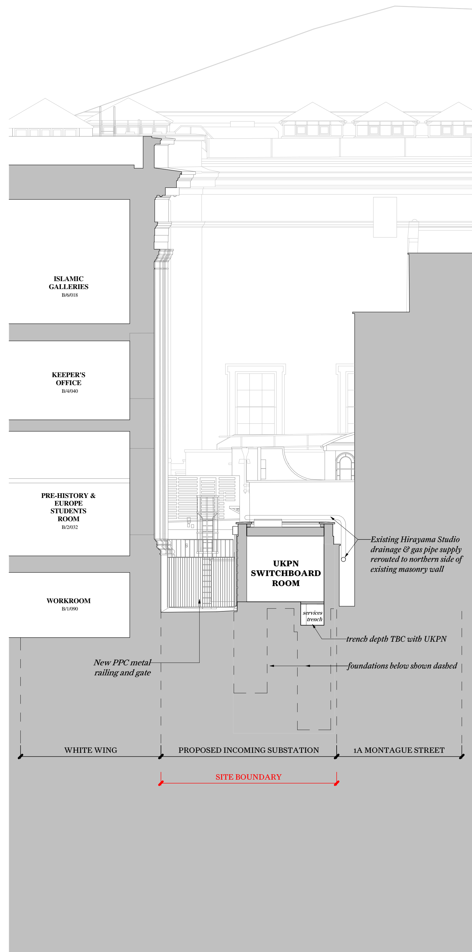
Proposed Section BB
