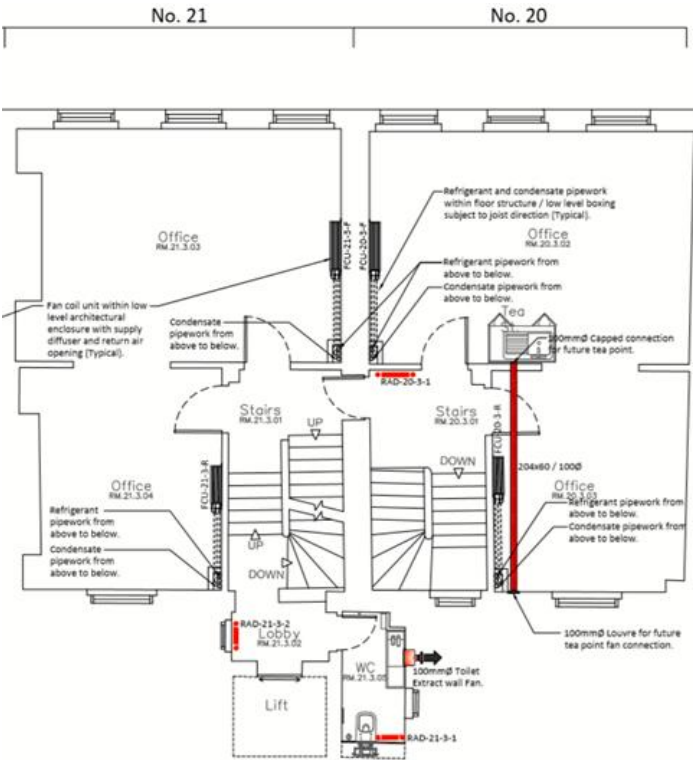
Figure 6 – Proposed Plant, Third Floor
