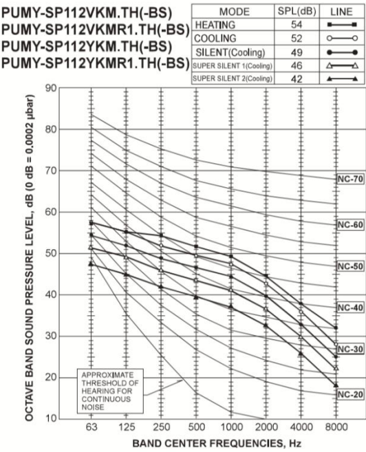
Figure 14 - Condensers
