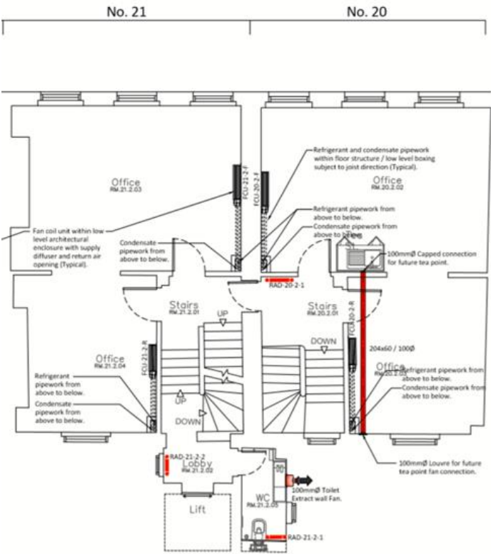
Figure 7 – Proposed Plant, Second Floor
