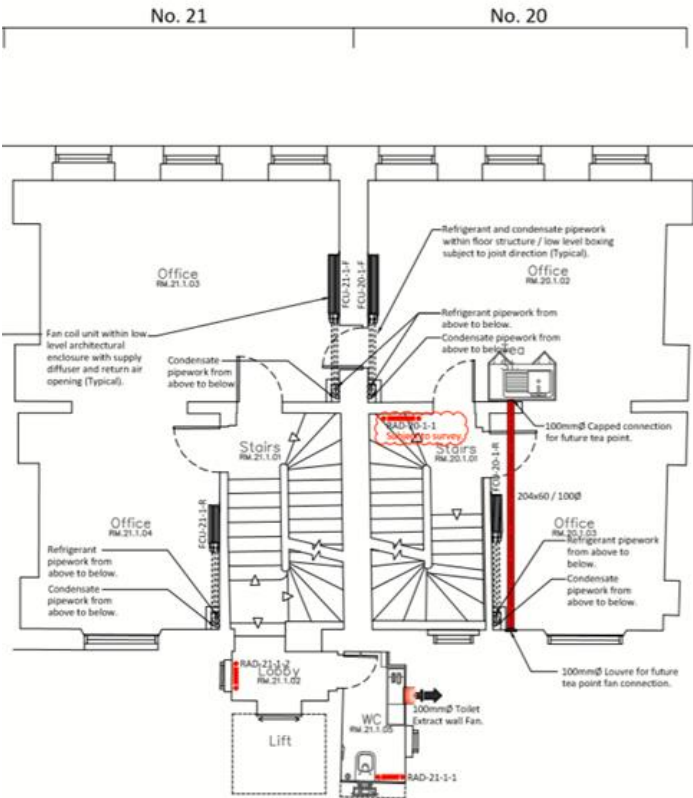
Figure 8 - Proposed Plant, First Floor
