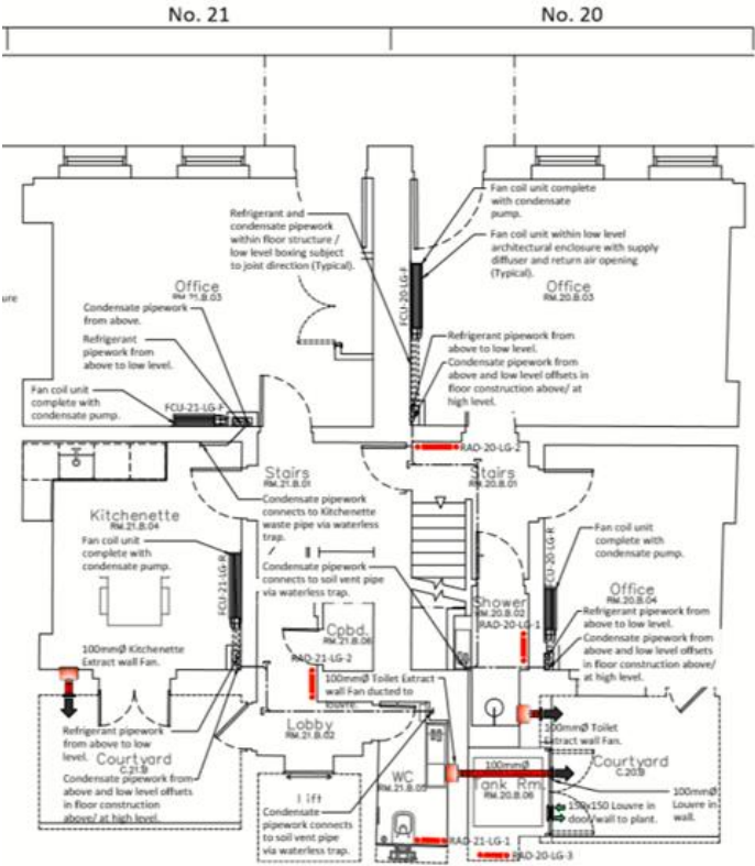
Figure 10 - Proposed Plant, Lower Ground Floor
