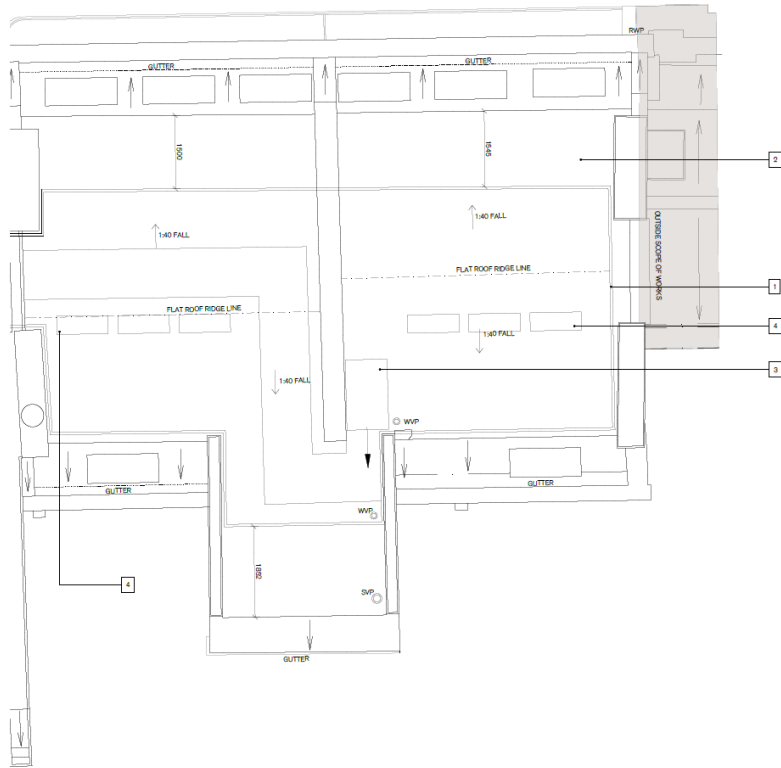
Figure 4 - Propose Plant, Roof Level
