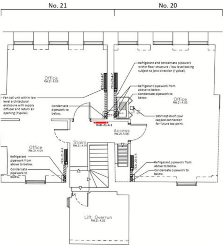
Figure 5 - Proposed Plant, Fourth Floor
