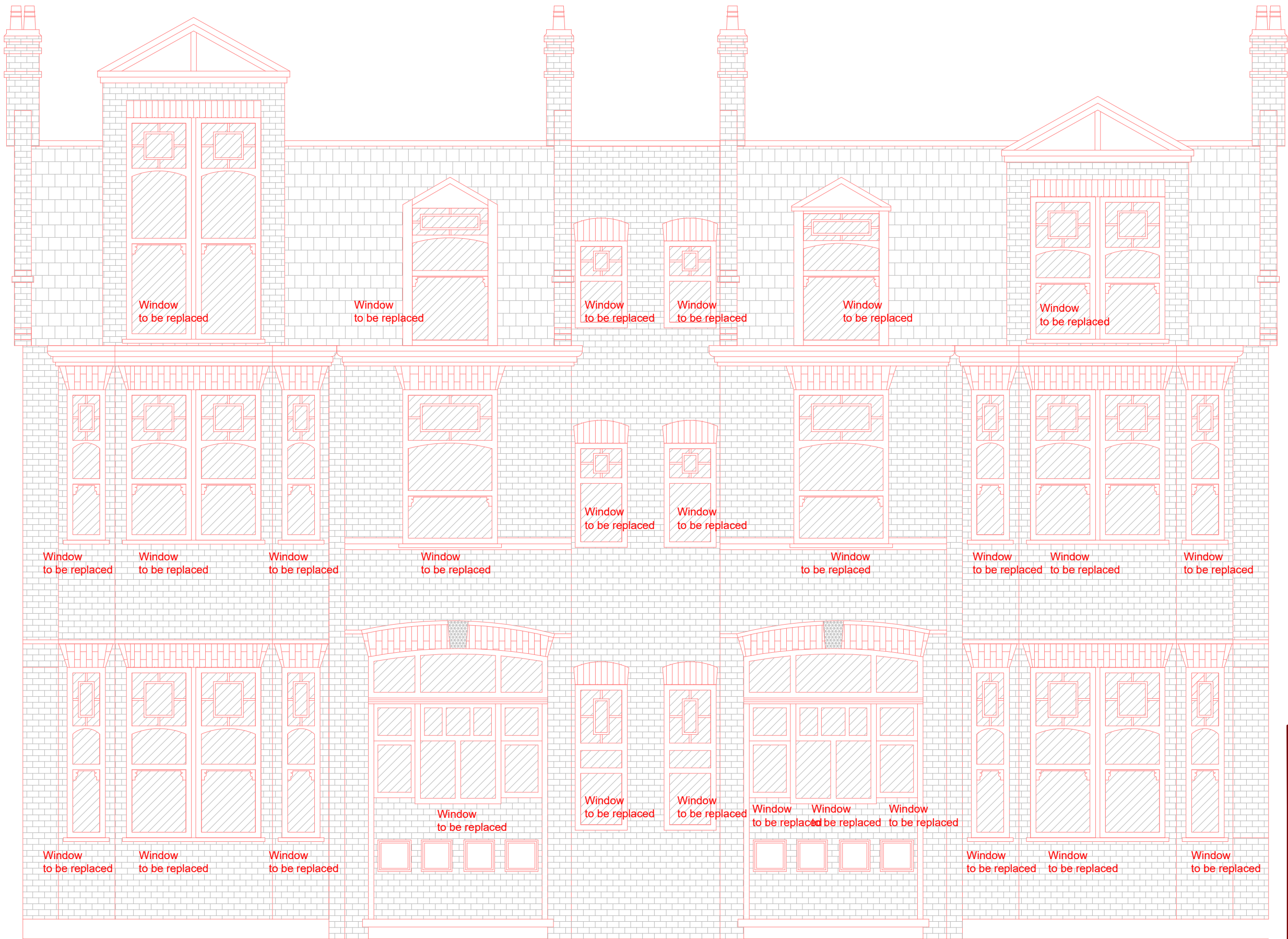
FRONT ELEVATION Scale 1:50
