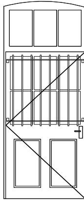
D01 (0031 - 2.01) Existing external glazed door Add traditional metal security bars
