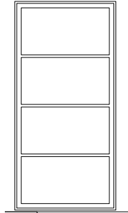
W02 New fixed window 996W x 1995H Aluminium frame
