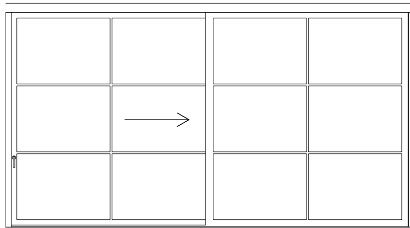
D06 (0031 - 2.02) New external sliding door 5220W x 2822H Aluminium frame
