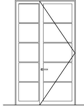
D03 (0031 - 2.01) New internal glazed partition and door 1377W x 2400H Steel frame
