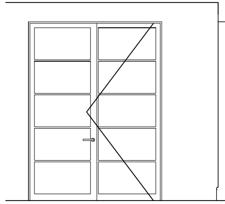
D02 (0031 - 2.01) New internal glazed partition and door 1800W x 2400H Steel frame Fire rated
