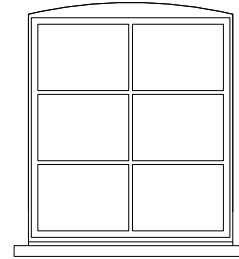
W05 Replacement side-hung casement 1351W x 1505H Aluminium frame
