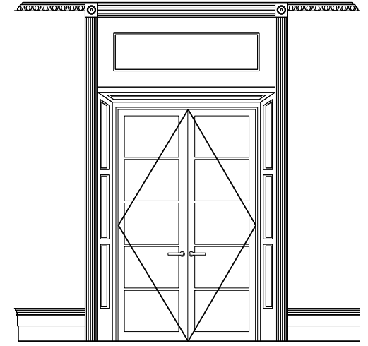
D05 (0031 - 2.02) New internal glazed doors 1327W x 2190H Steel frame Fire rated
