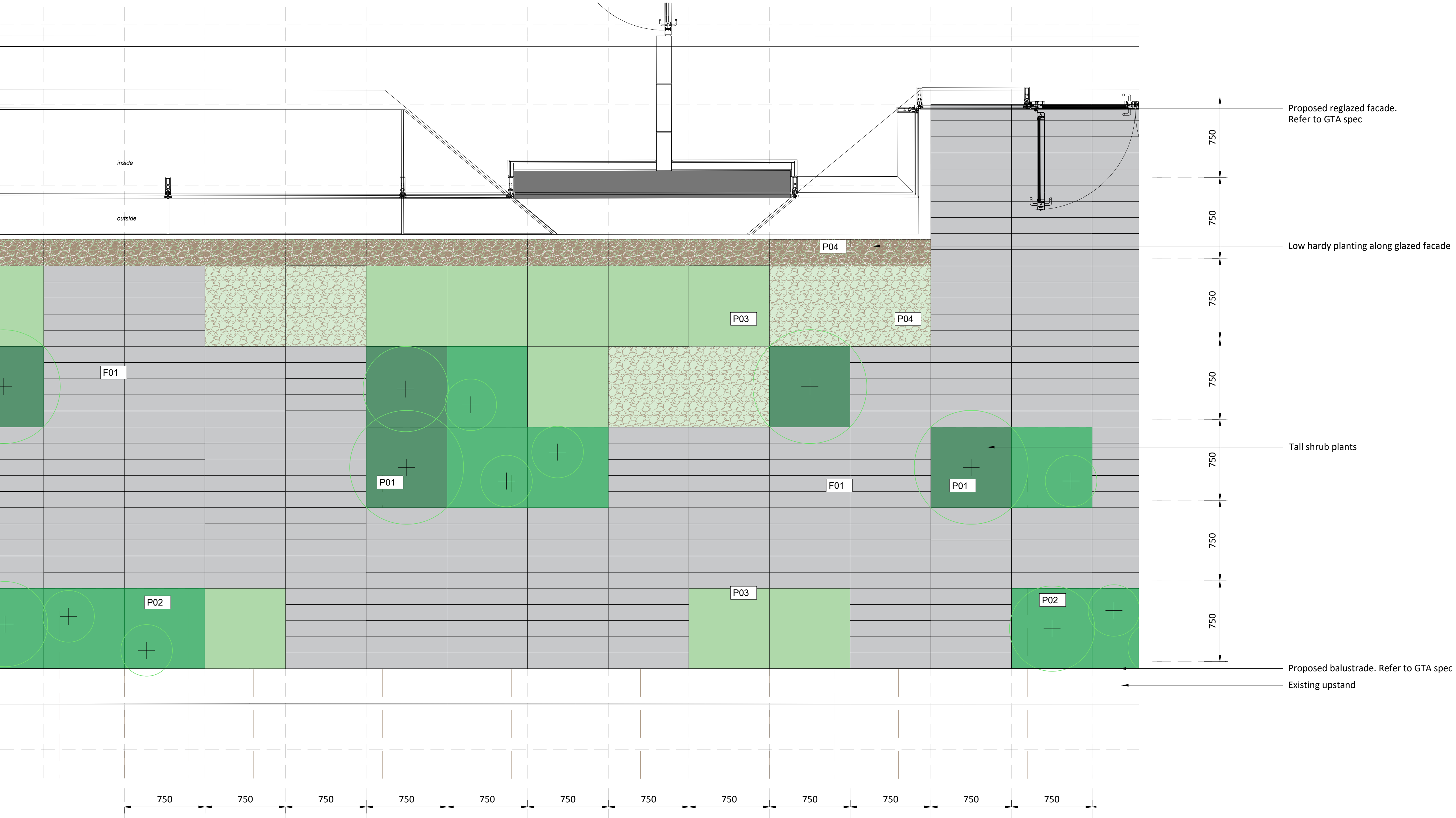
2 L08 Block A Terrace - Detail Plan 1:20
