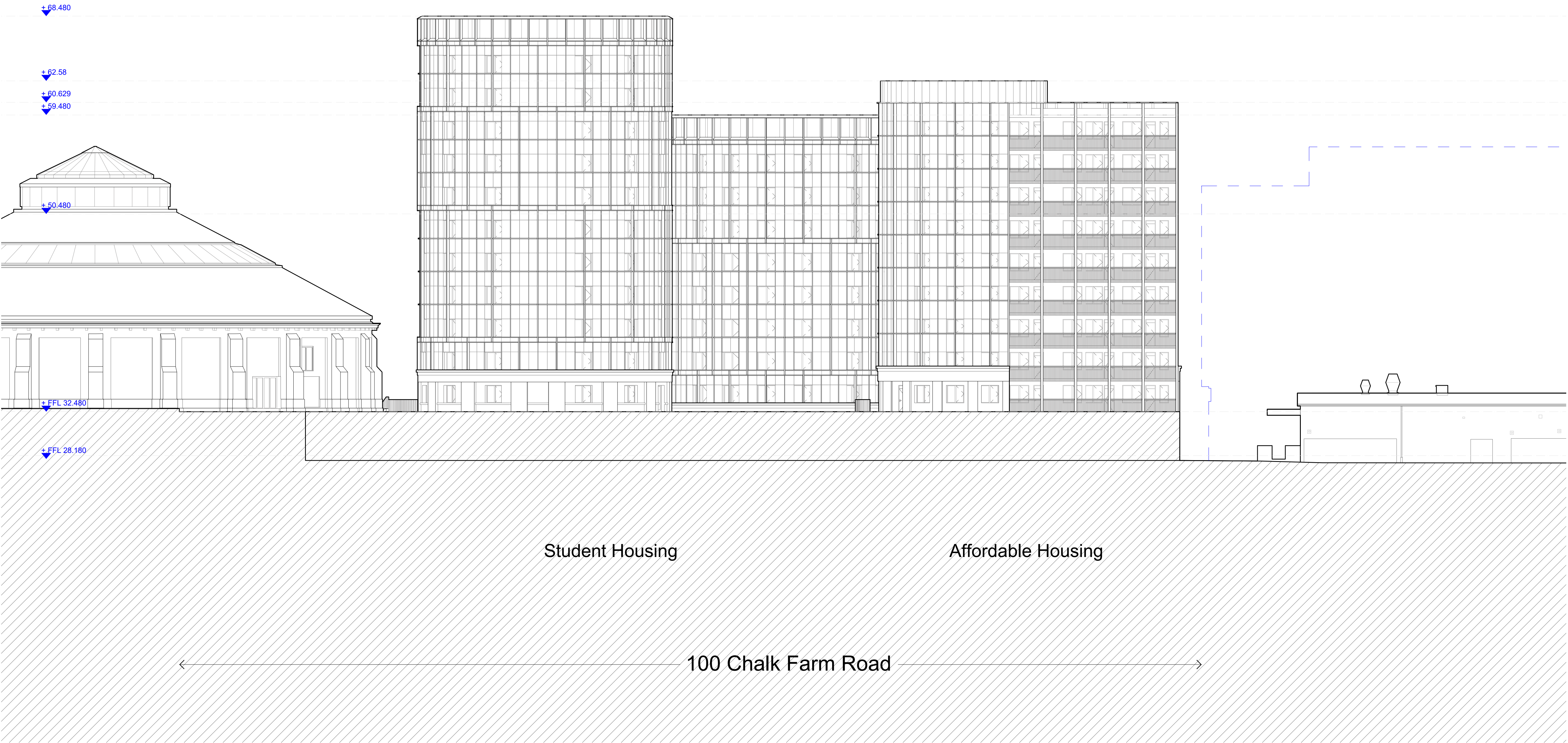
Proposed South Elevation
