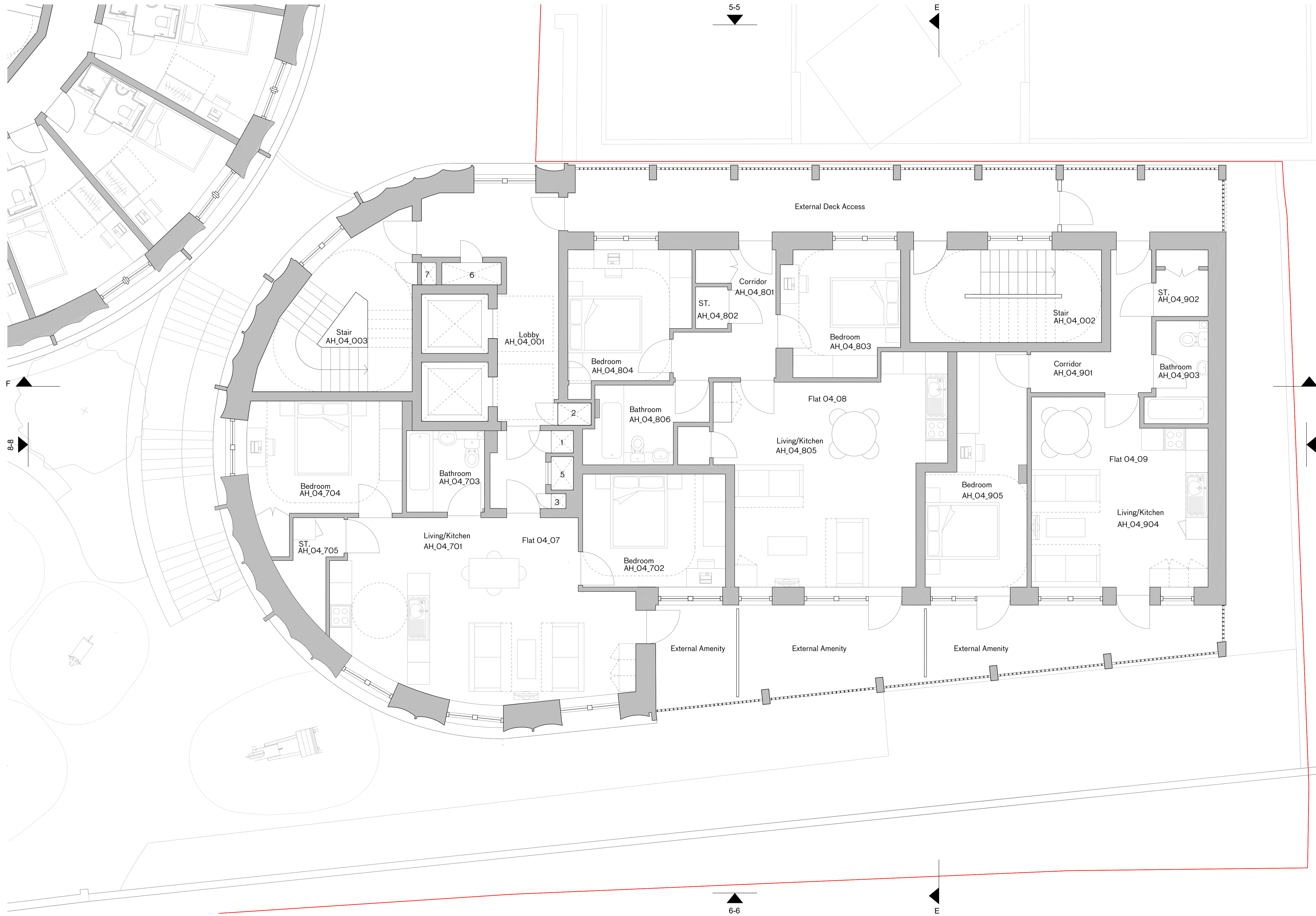
Affordable Housing Level 4 - 5 Floor Plan
