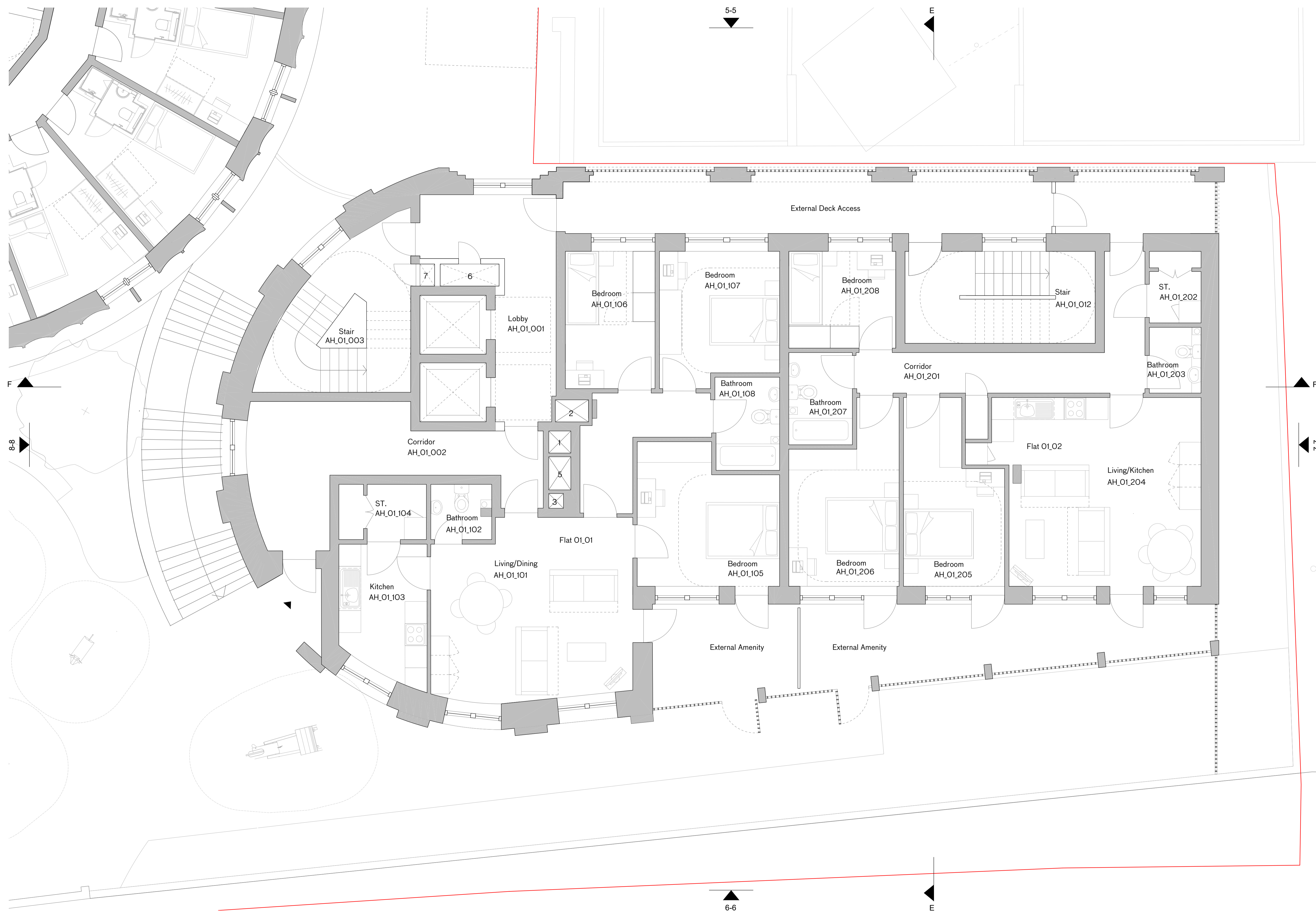
Affordable Housing Level 1 Floor Plan
