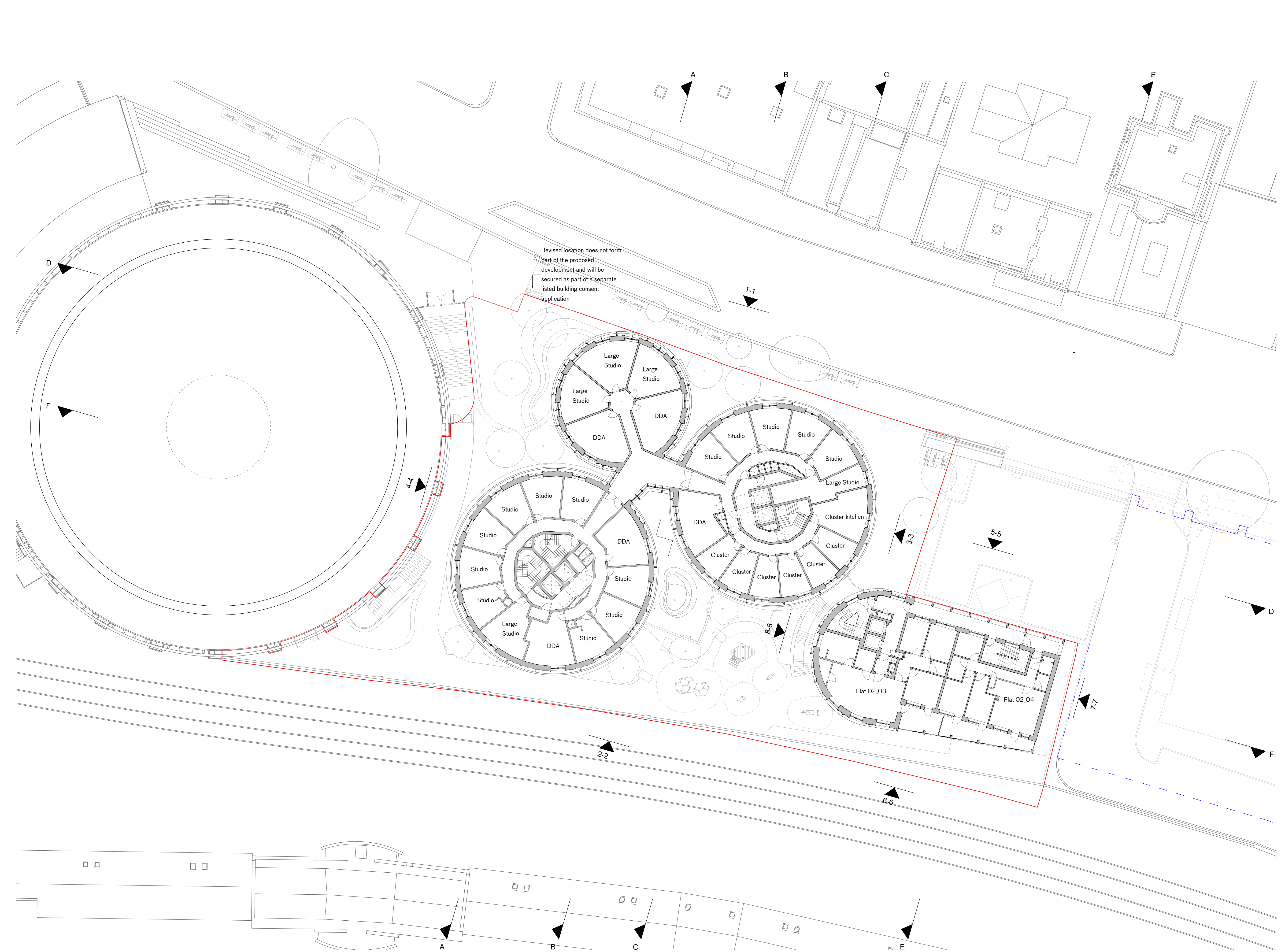
Level 2 - 3 Floor Plan
