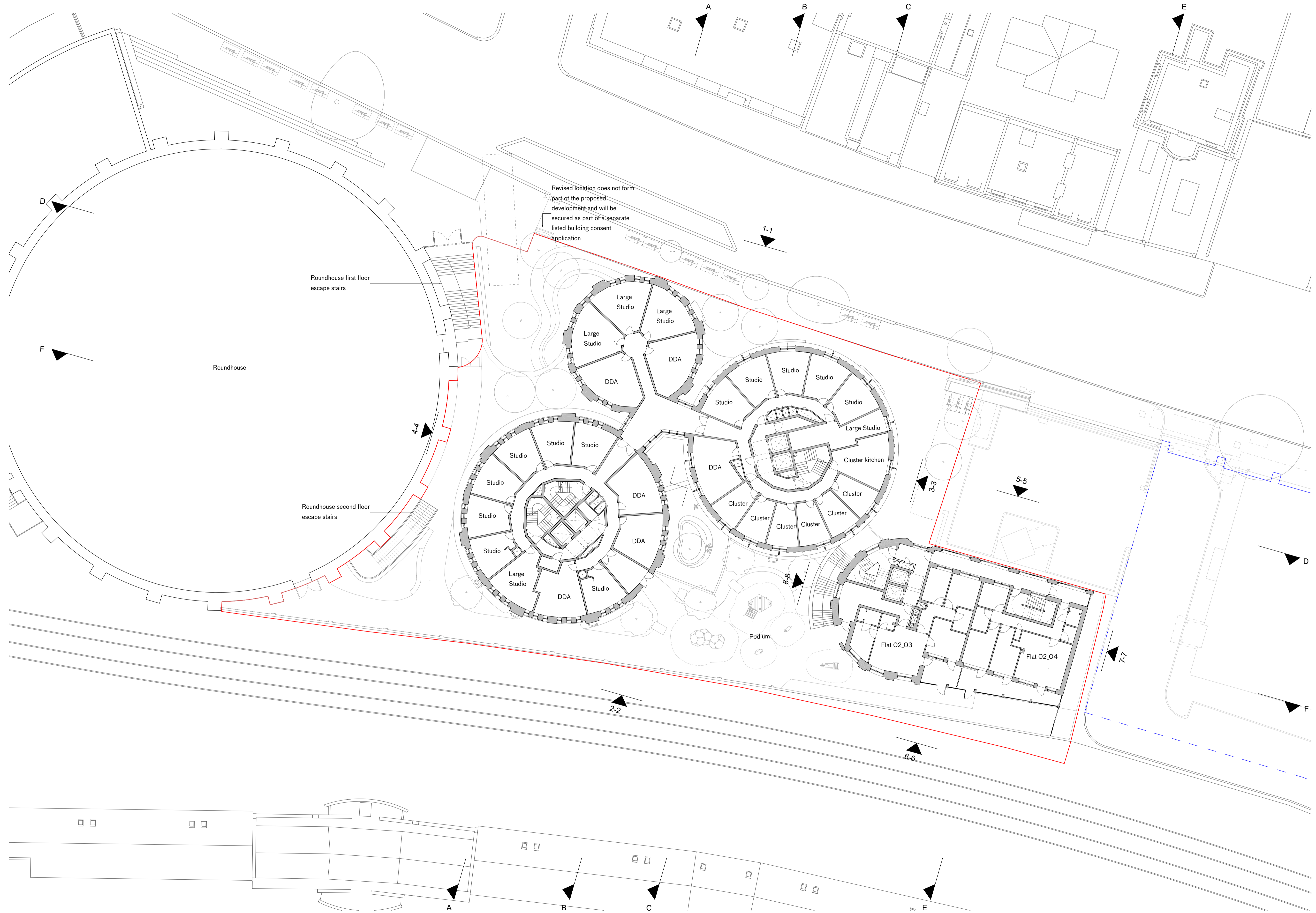
Level 1 Floor Plan
