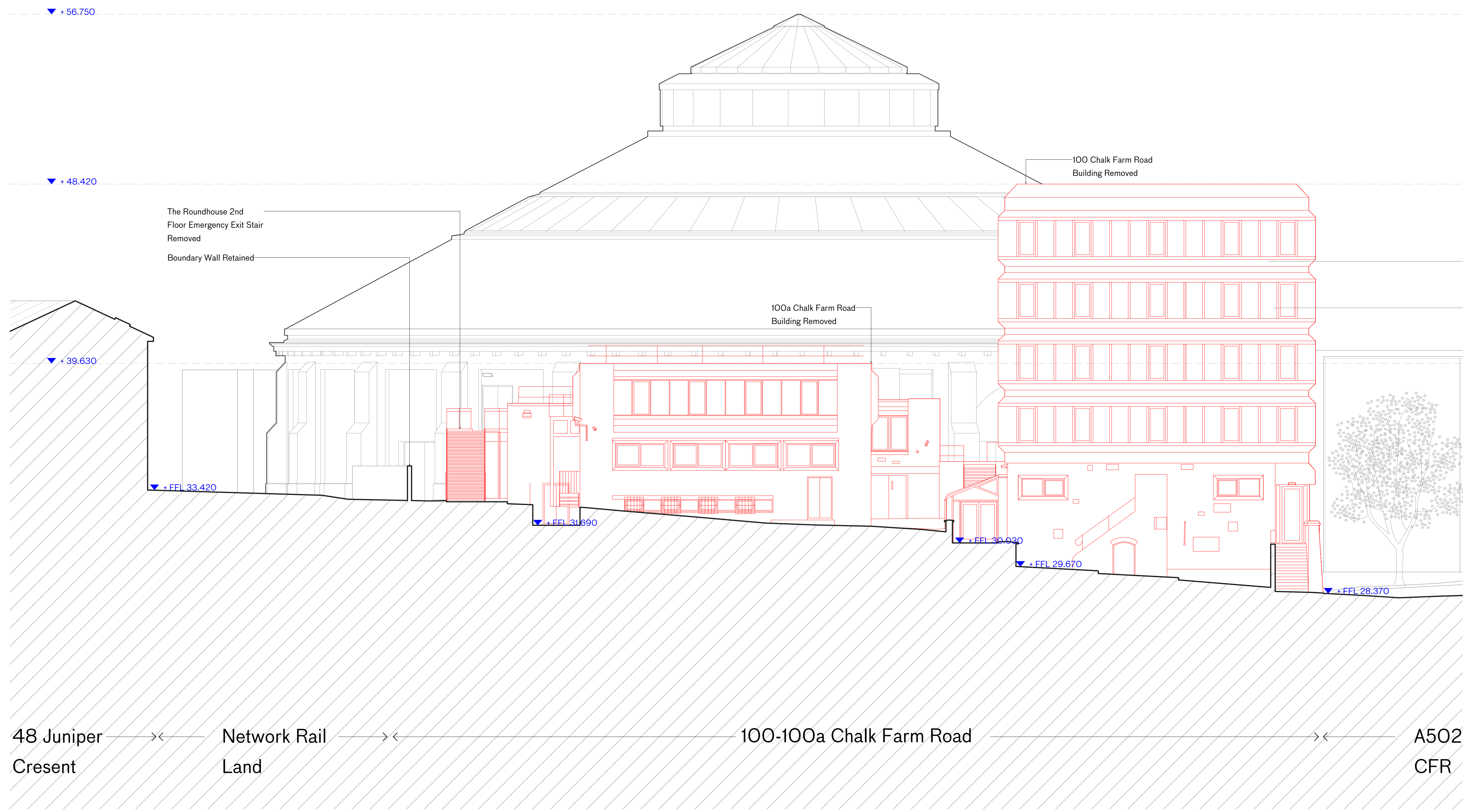
Demolition Elevation 3 - 3 East
