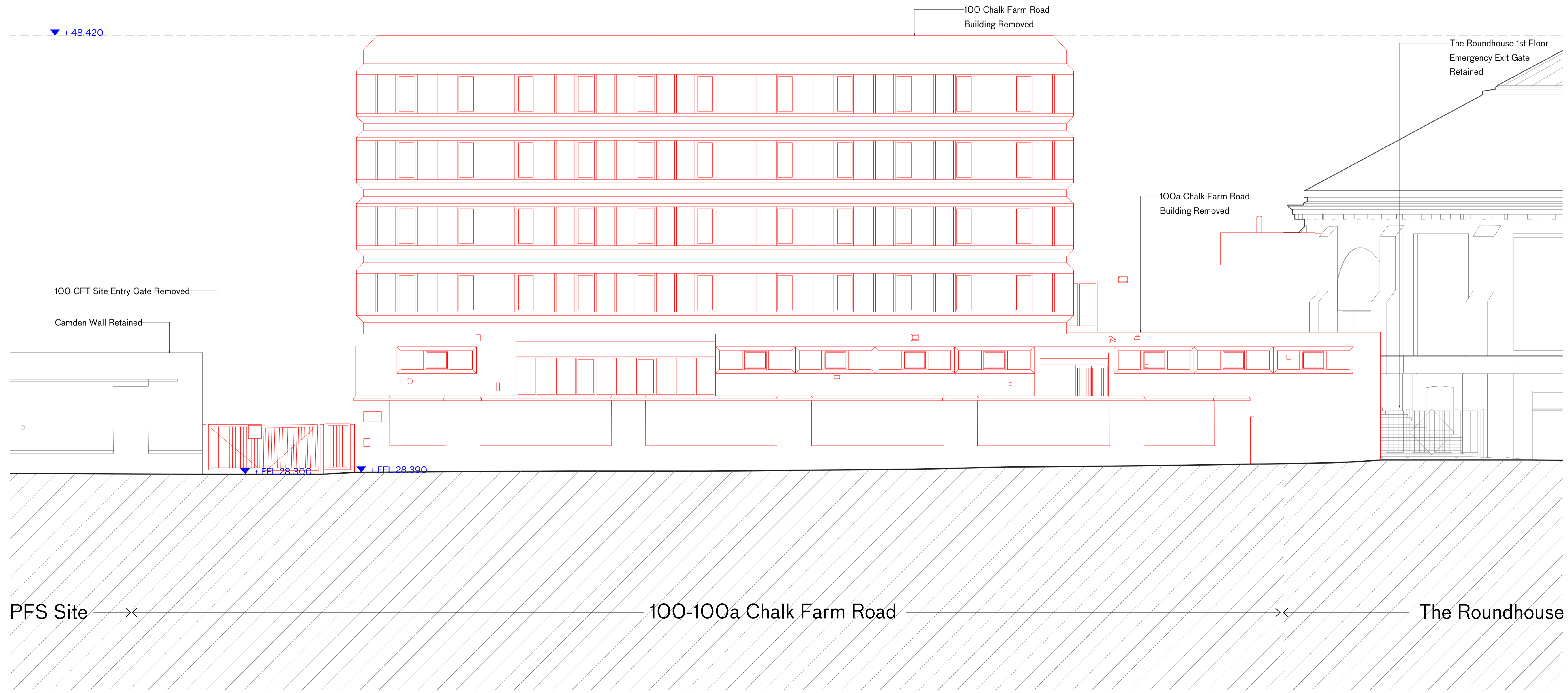
Demolition Elevation 1 - 1 North
