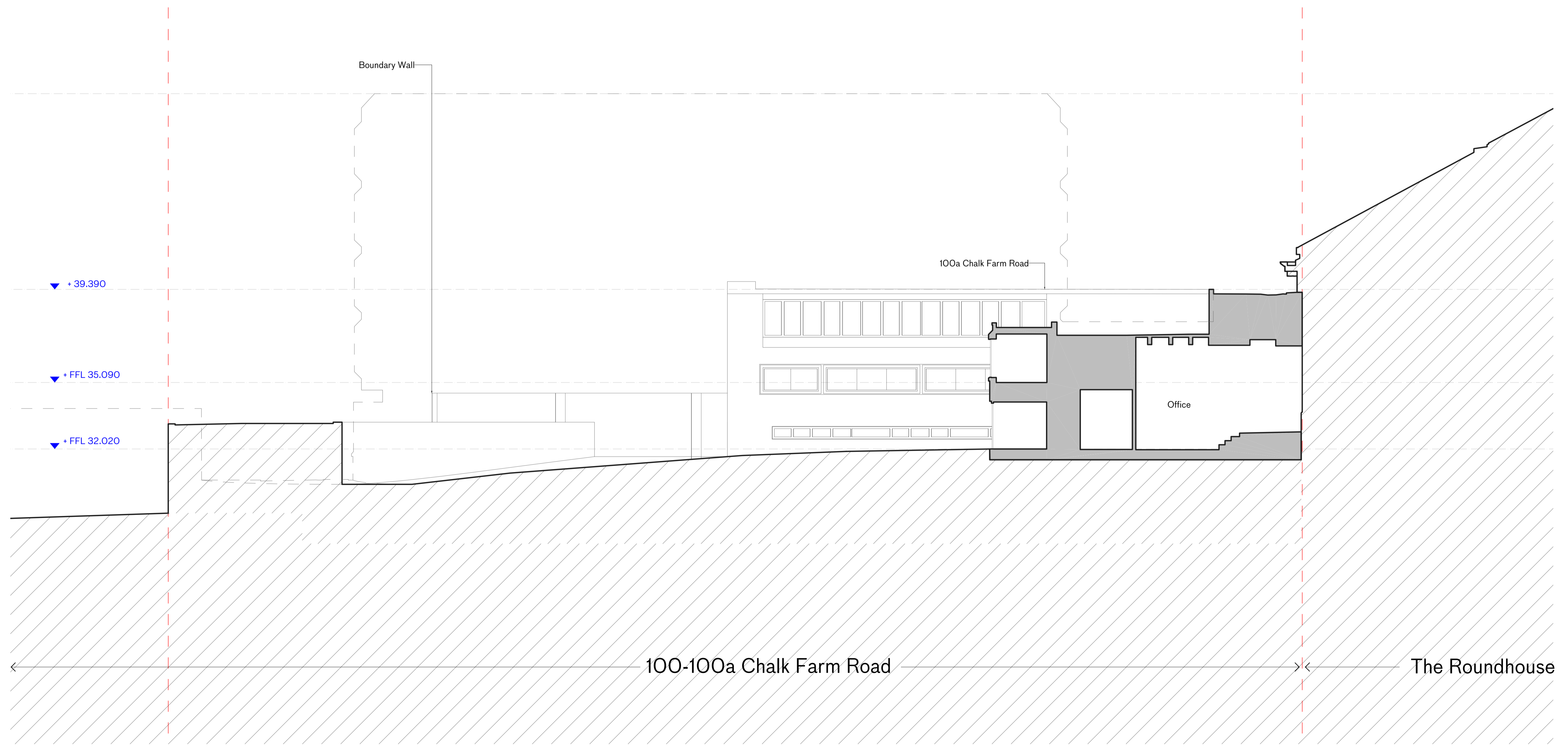
Existing Section BB
