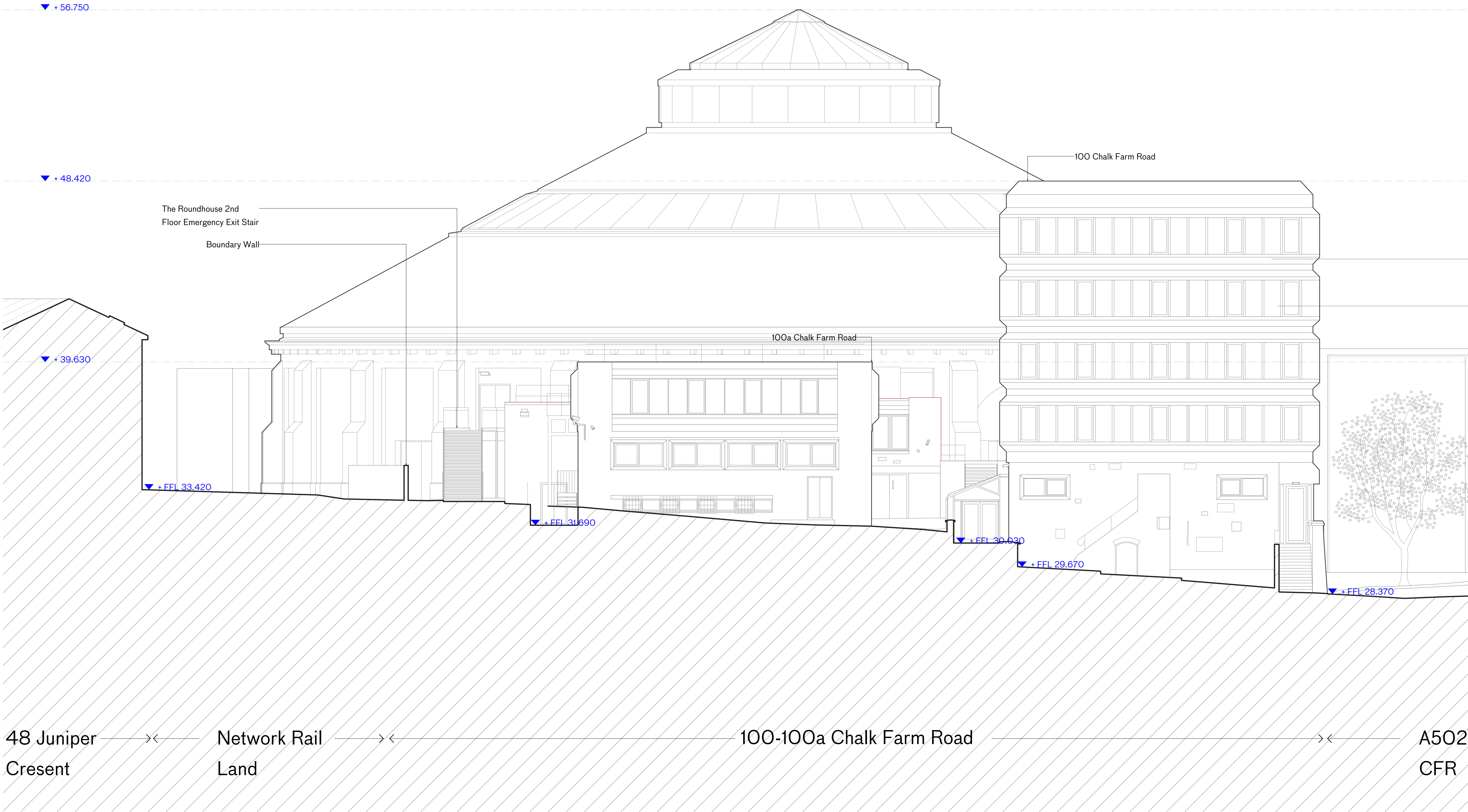
Existing Elevation 3 - 3 East
