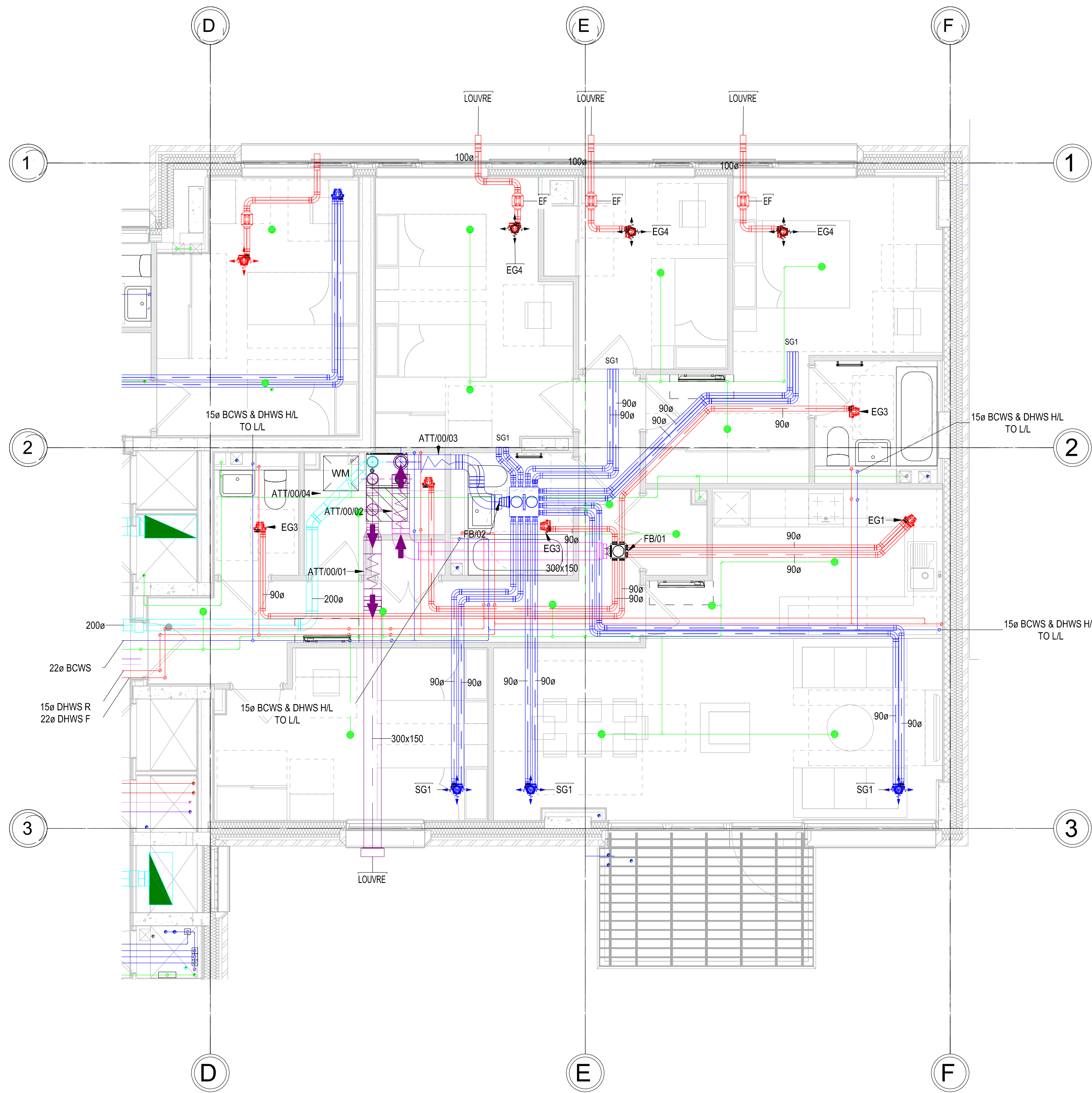
05 - Typical Apartment Type G - H/L
