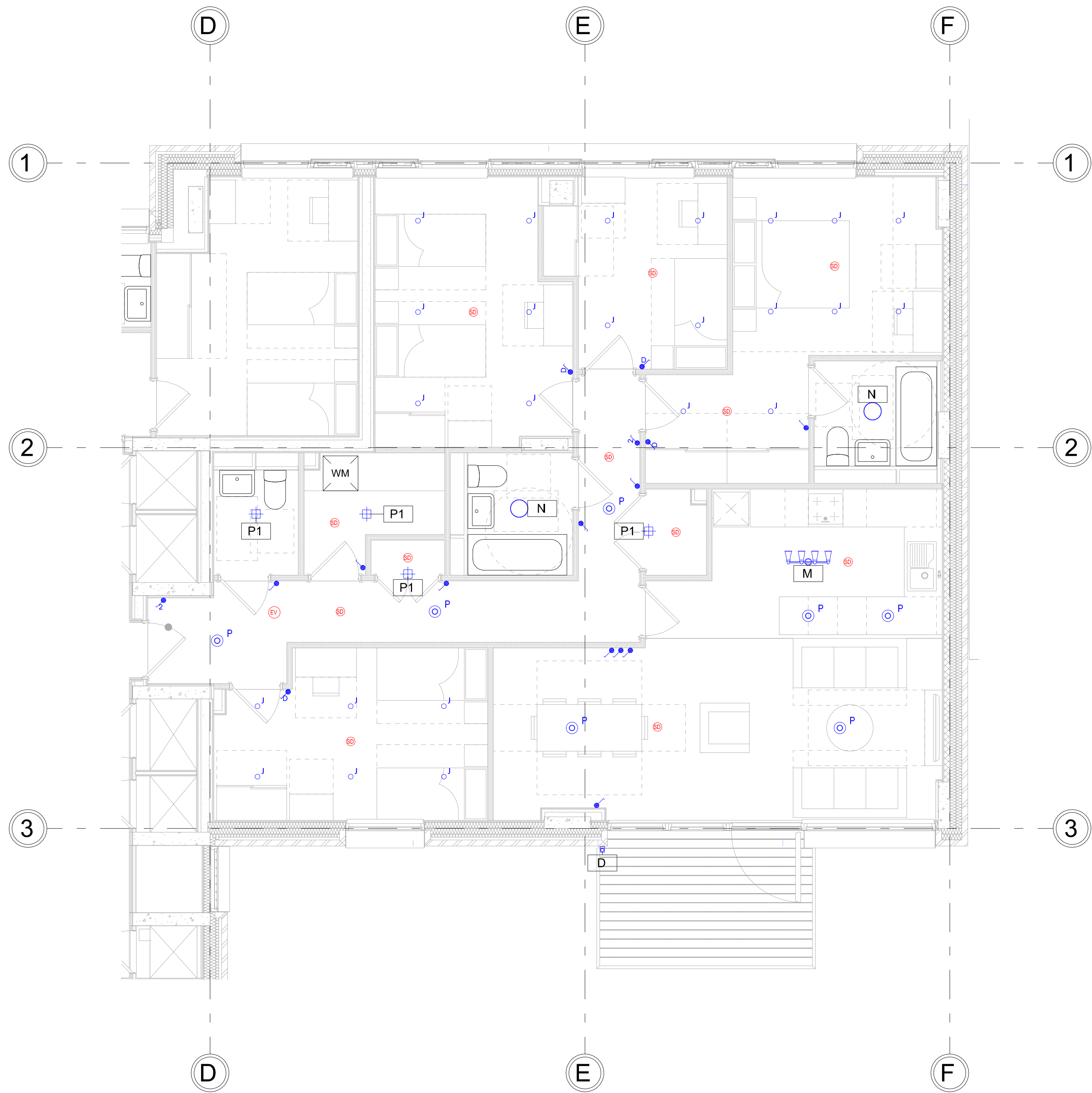
05 - Typical Apartment Type G - Lighting and FA
