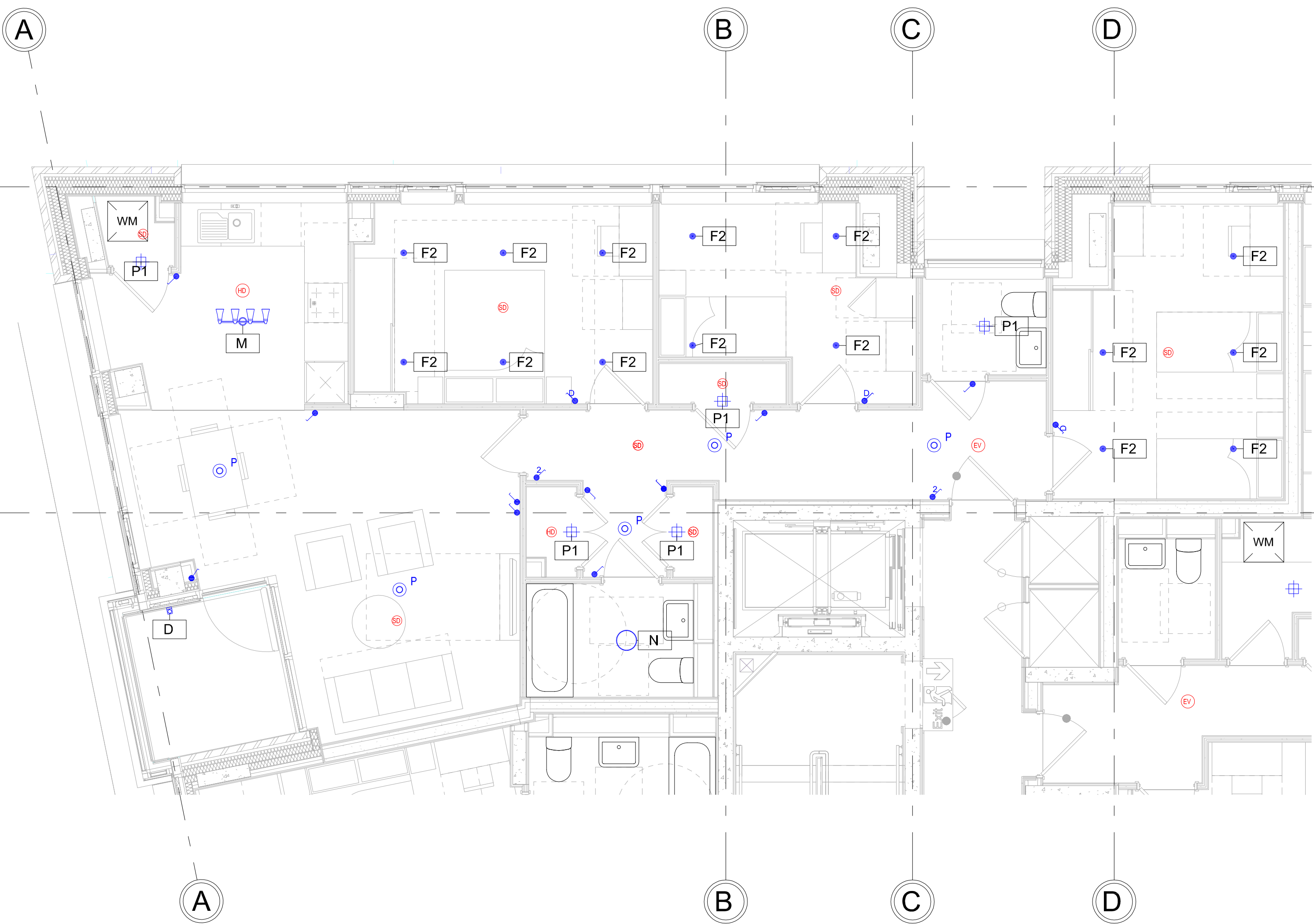
05 - Typical Apartment Type F - Lighting and FA
