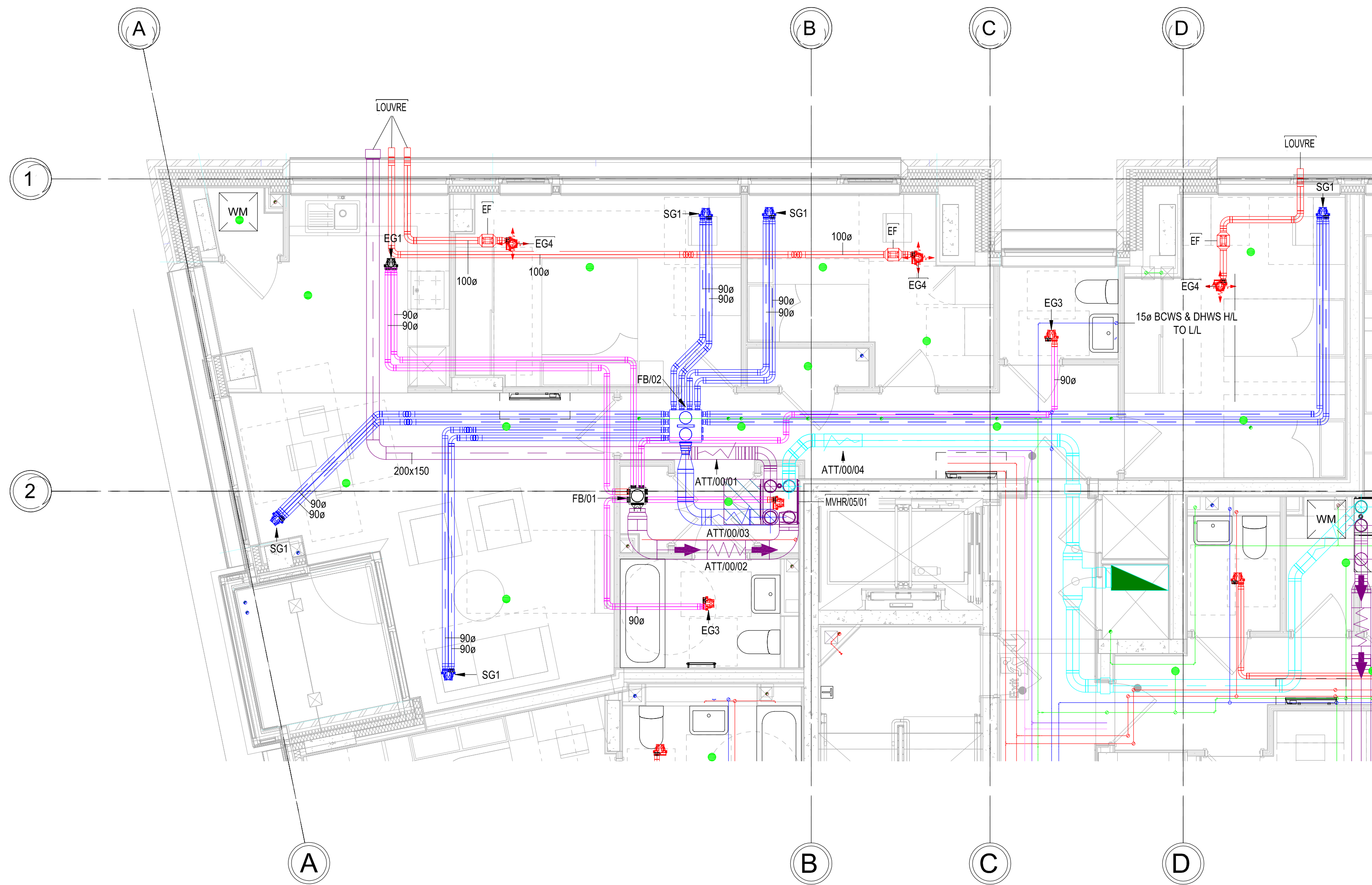
05 - Typical Apartment Type F - H/L
