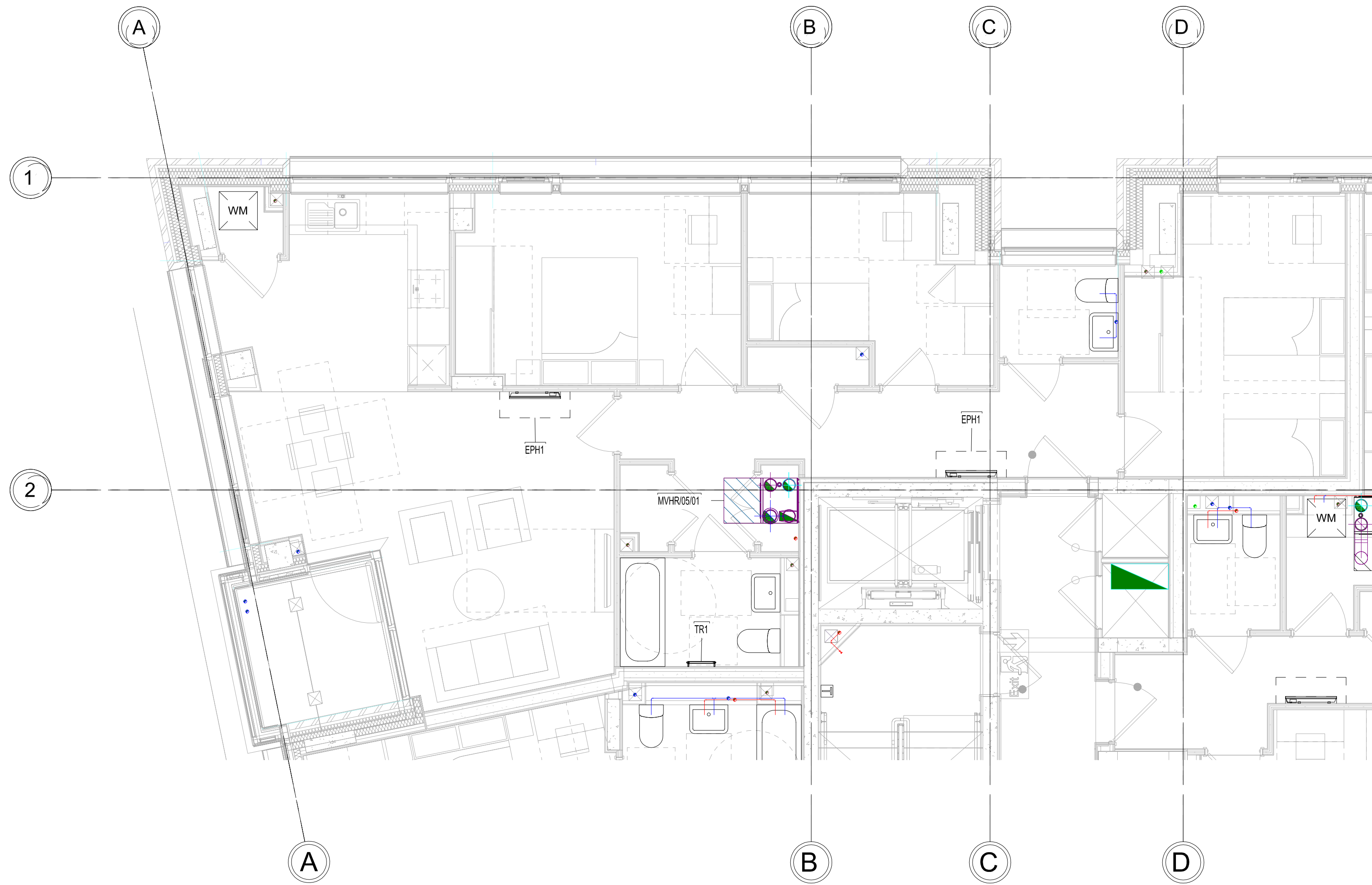
05 - Typical Apartment Type F - L/L
