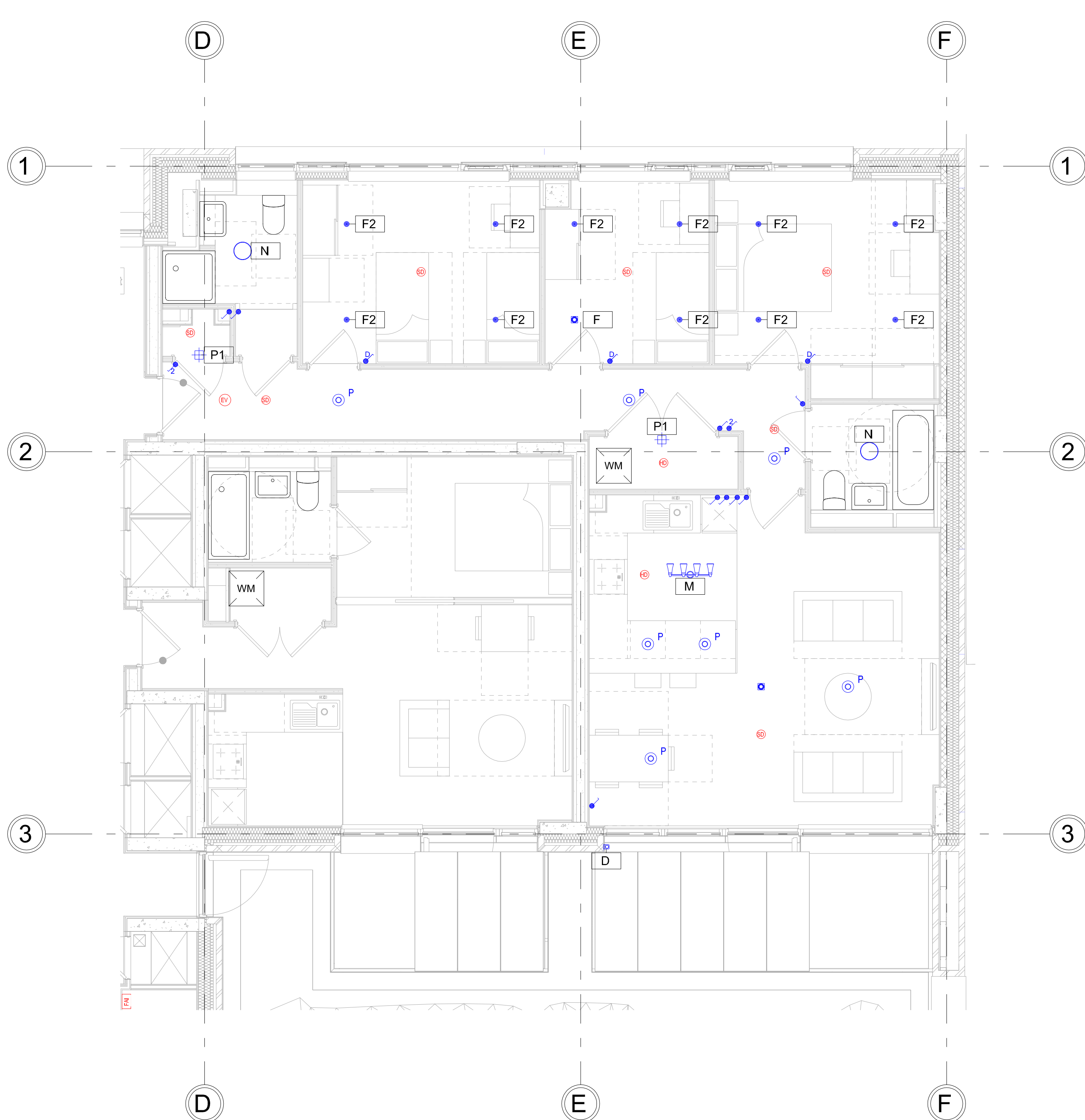
01 - Typical Apartment Type E - Lighting and FA 1 : 50
