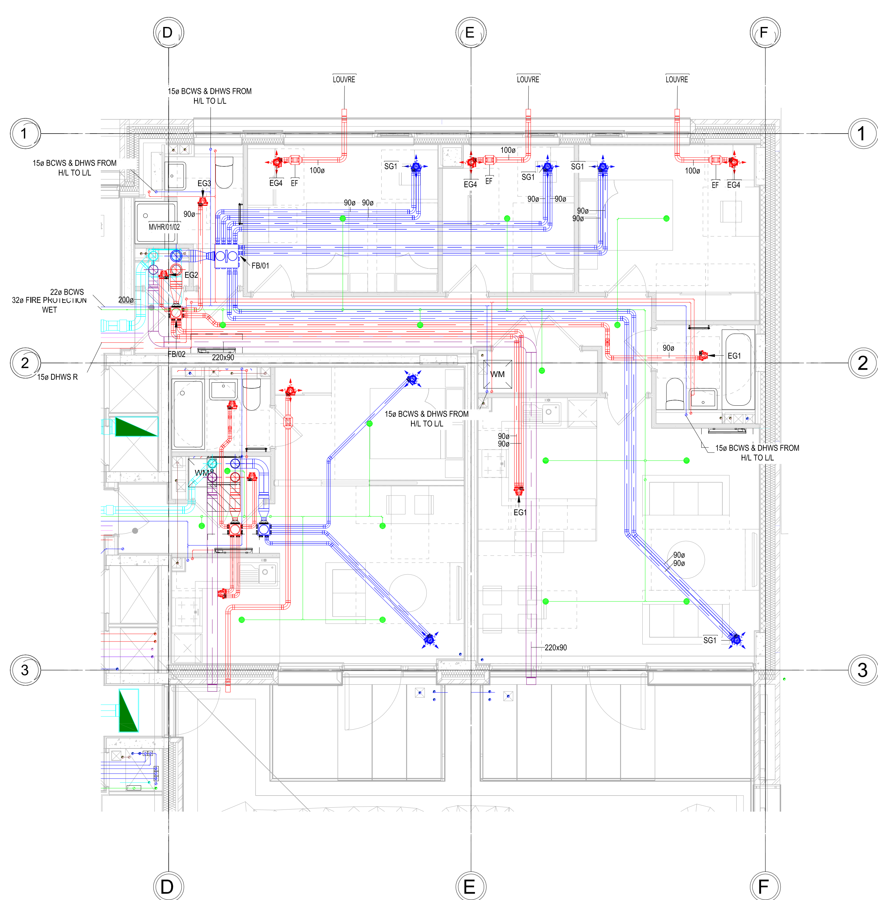
01 - Typical Apartment Type E - H/L 1 : 50
