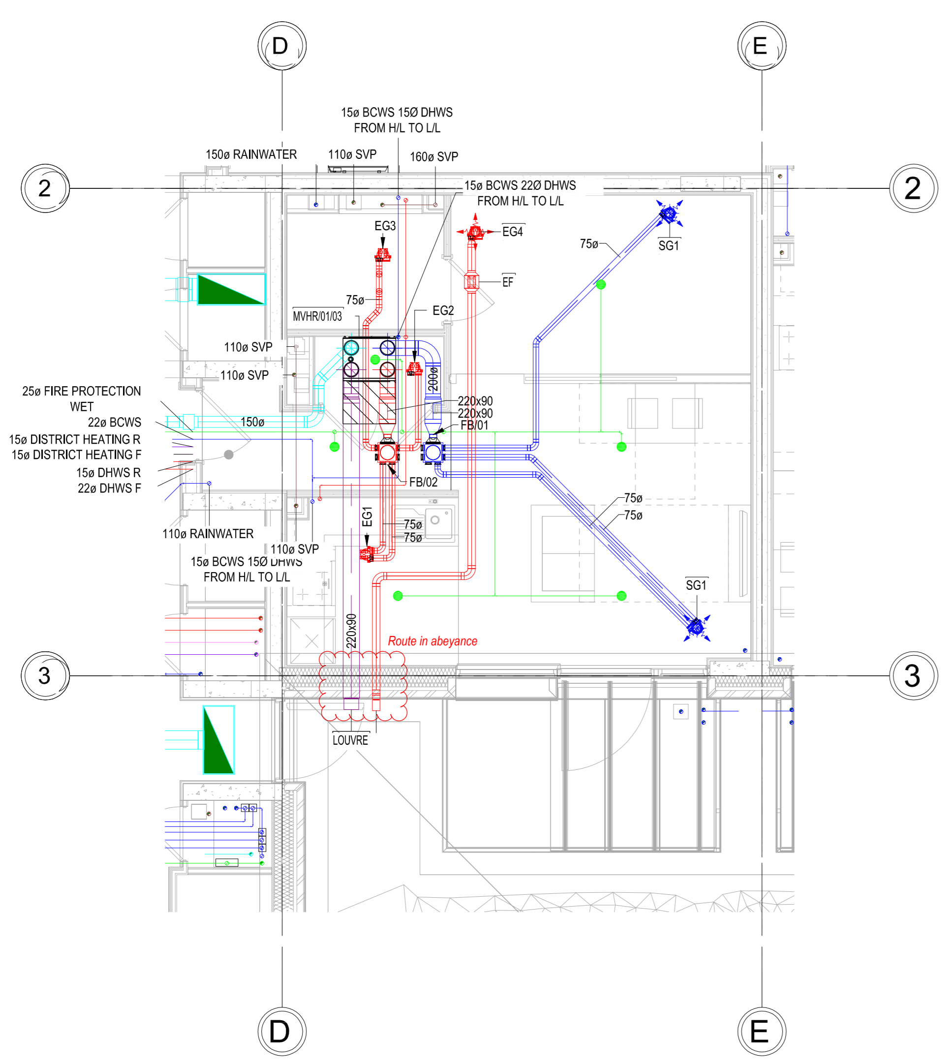
○ 01 - Typical Apartment Type A - H/L 1 : 50
