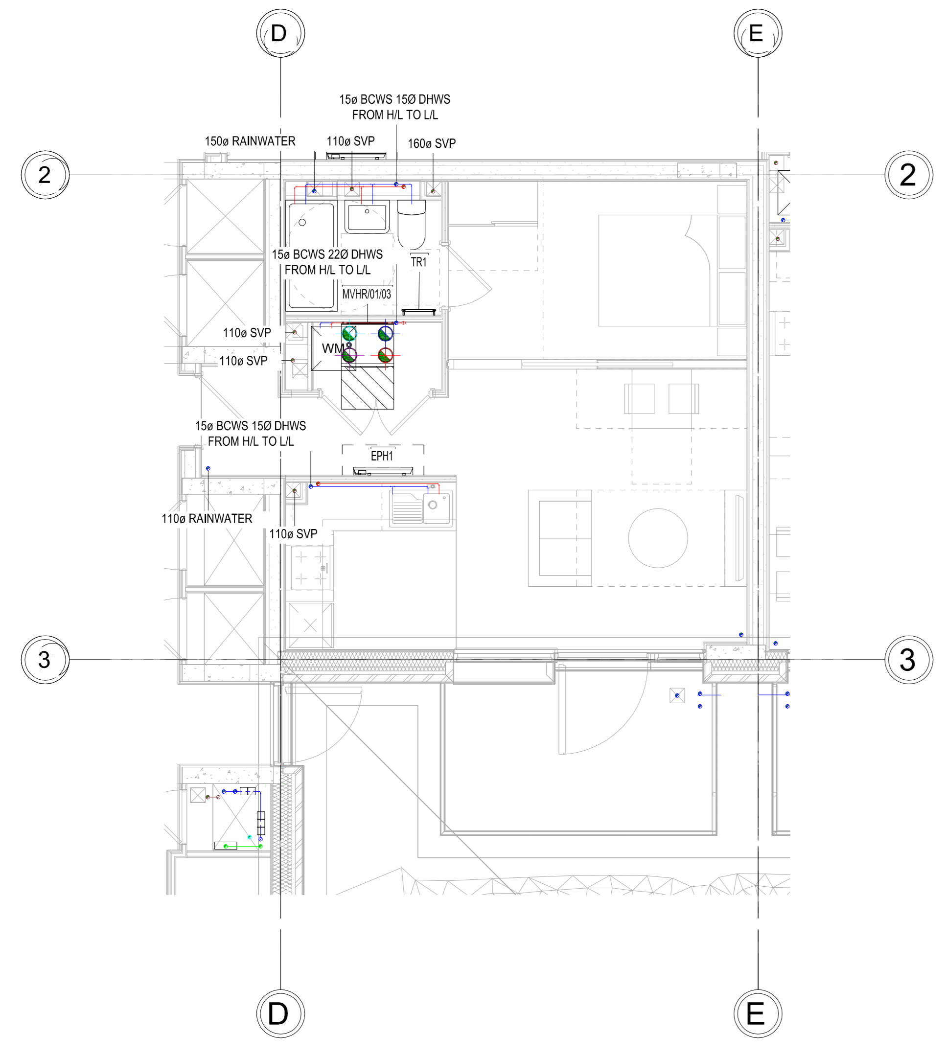
○ 01 - Typical Apartment Type A - L/L 1 : 50
