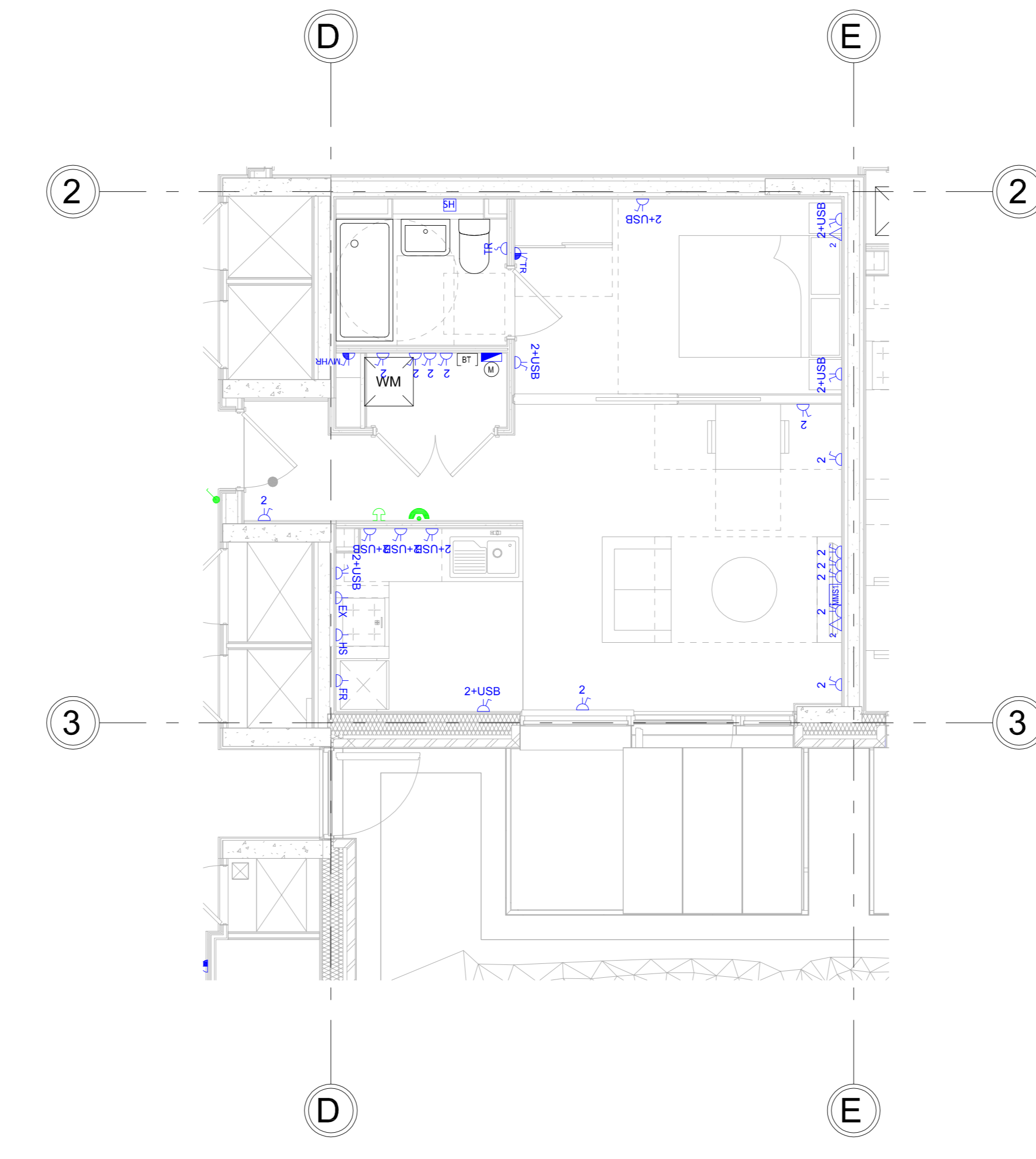
○ 01 - Typical Apartment Type A - Small Power and AC 1 : 50
