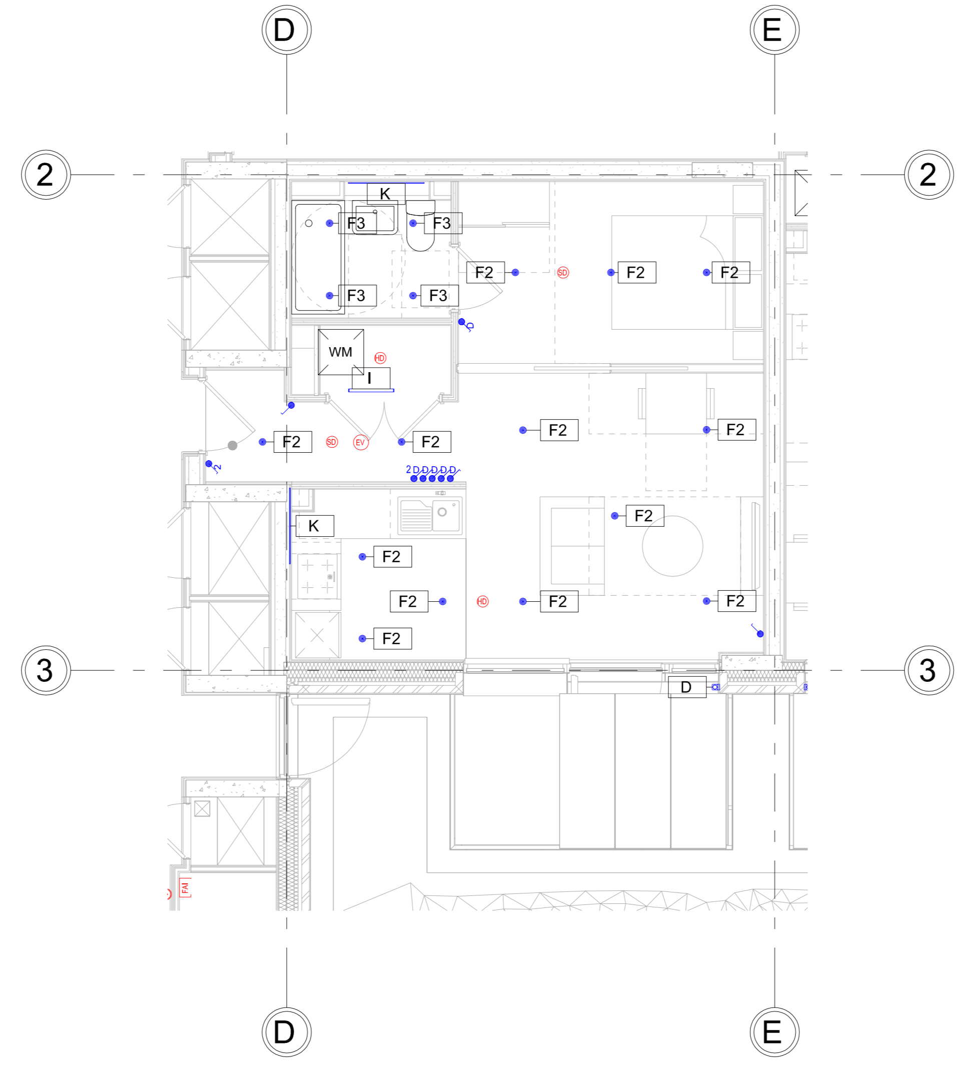
○ 01 - Typical Apartment Type A - Lighting and FA 1 : 50
