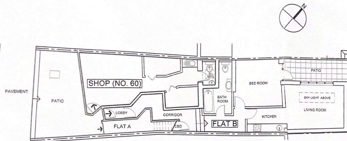
GENERAL ARRANGEMENT - GROUND FLOOR SCALE 1:100
