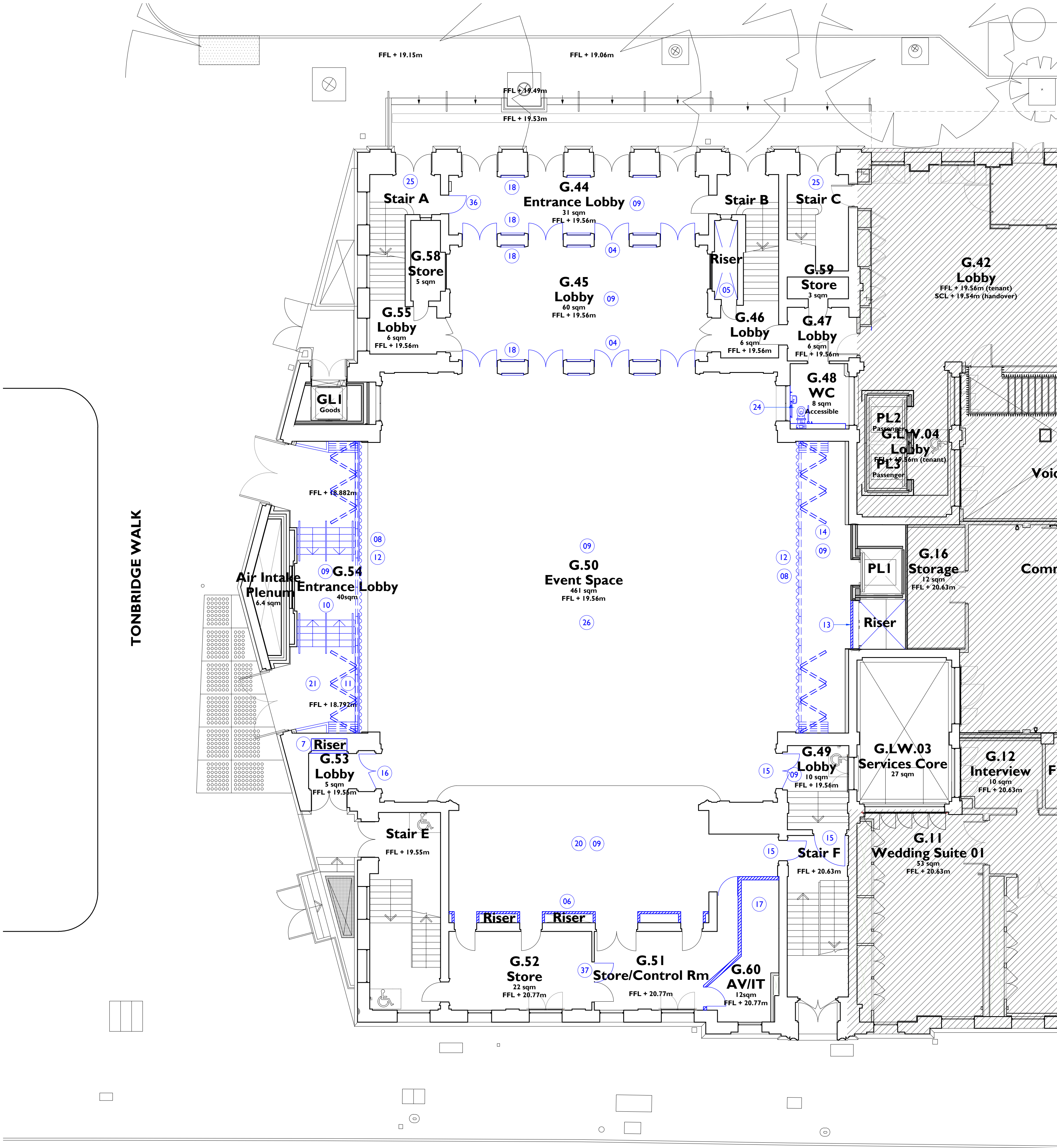
1 PROPOSED CAMDEN CENTRE GROUND FLOOR PLAN 4001 1:100 @ A1
