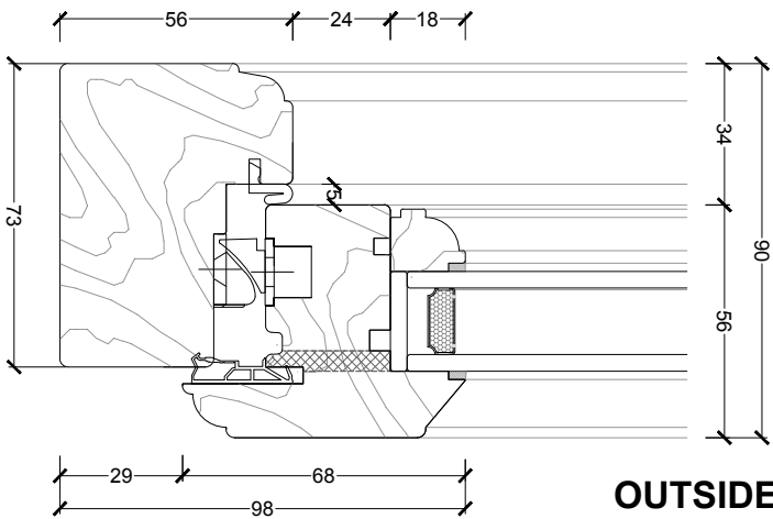
DORMER WINDOW SECTION BB' 1:2@A3
