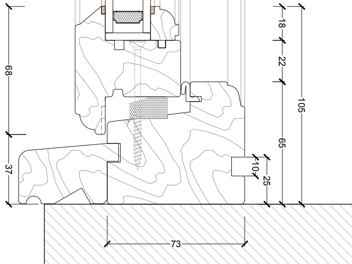
DORMER WINDOW SECTION AA' 1:2@A3
