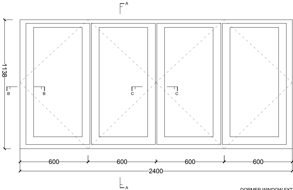
DORMER WINDOW EXTERNAL ELEVATION 1:20@A3
