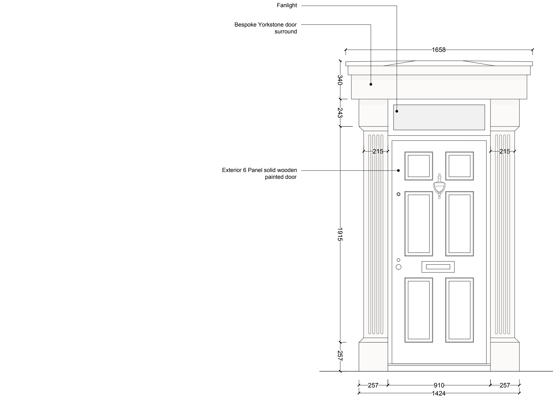
PROPOSED FRONT DOOR AND DOOR SURROUND EXTERNAL VIEW 1:20@A3
