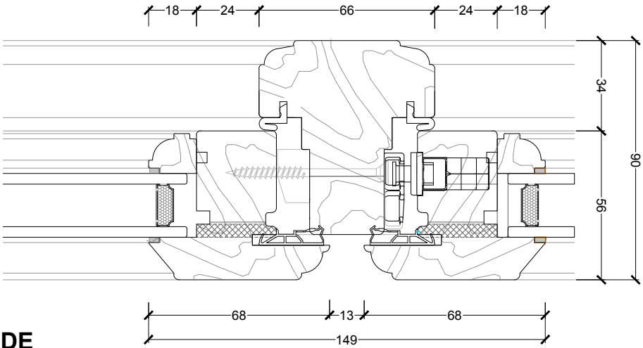
DORMER WINDOW SECTION CC' 1:2@A3
