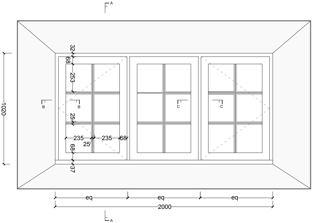
DORMER WINDOW EXTERNAL ELEVATION 1:20@A3
