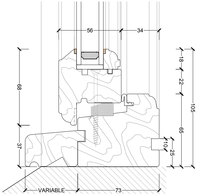
DORMER WINDOW SECTION AA' 1:2@A3
