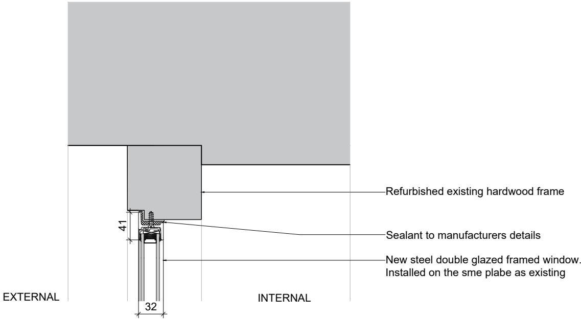
2. TYPICAL HEAD DETAIL
