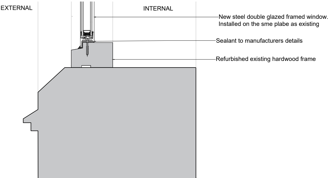
3. TYPICAL CILL DETAIL
