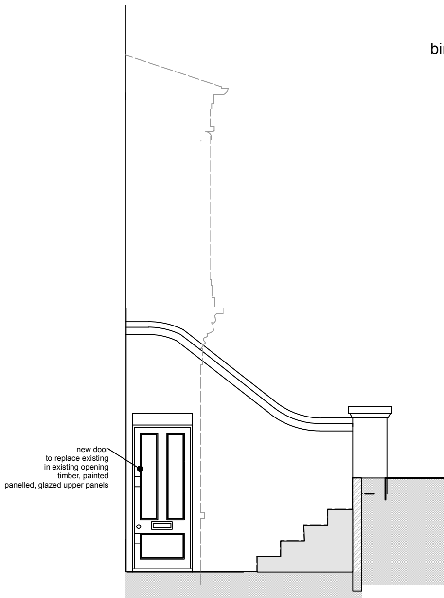
LGF entrance door elevation - proposed
