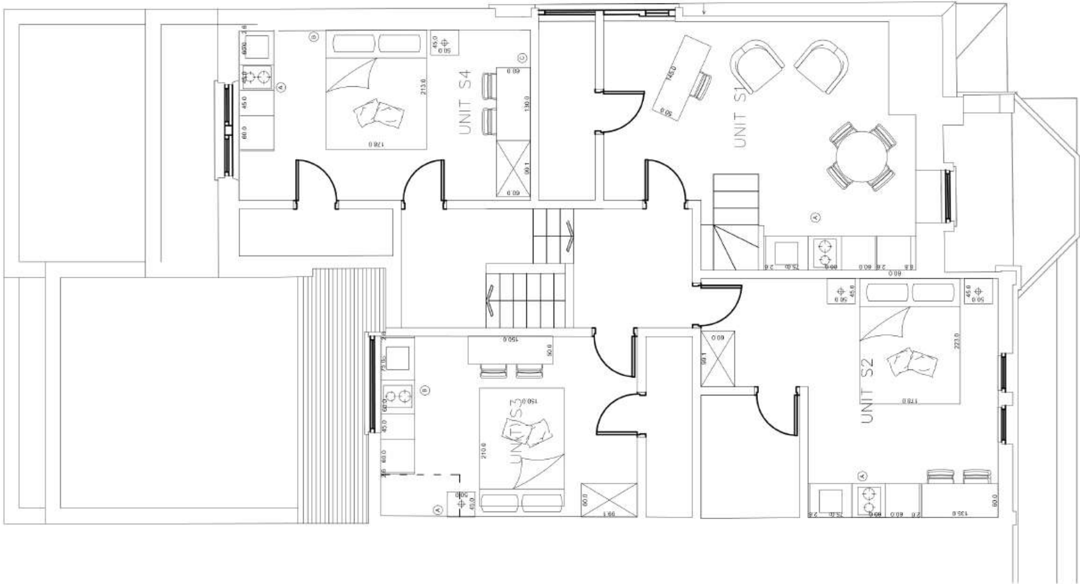
Second Floor
