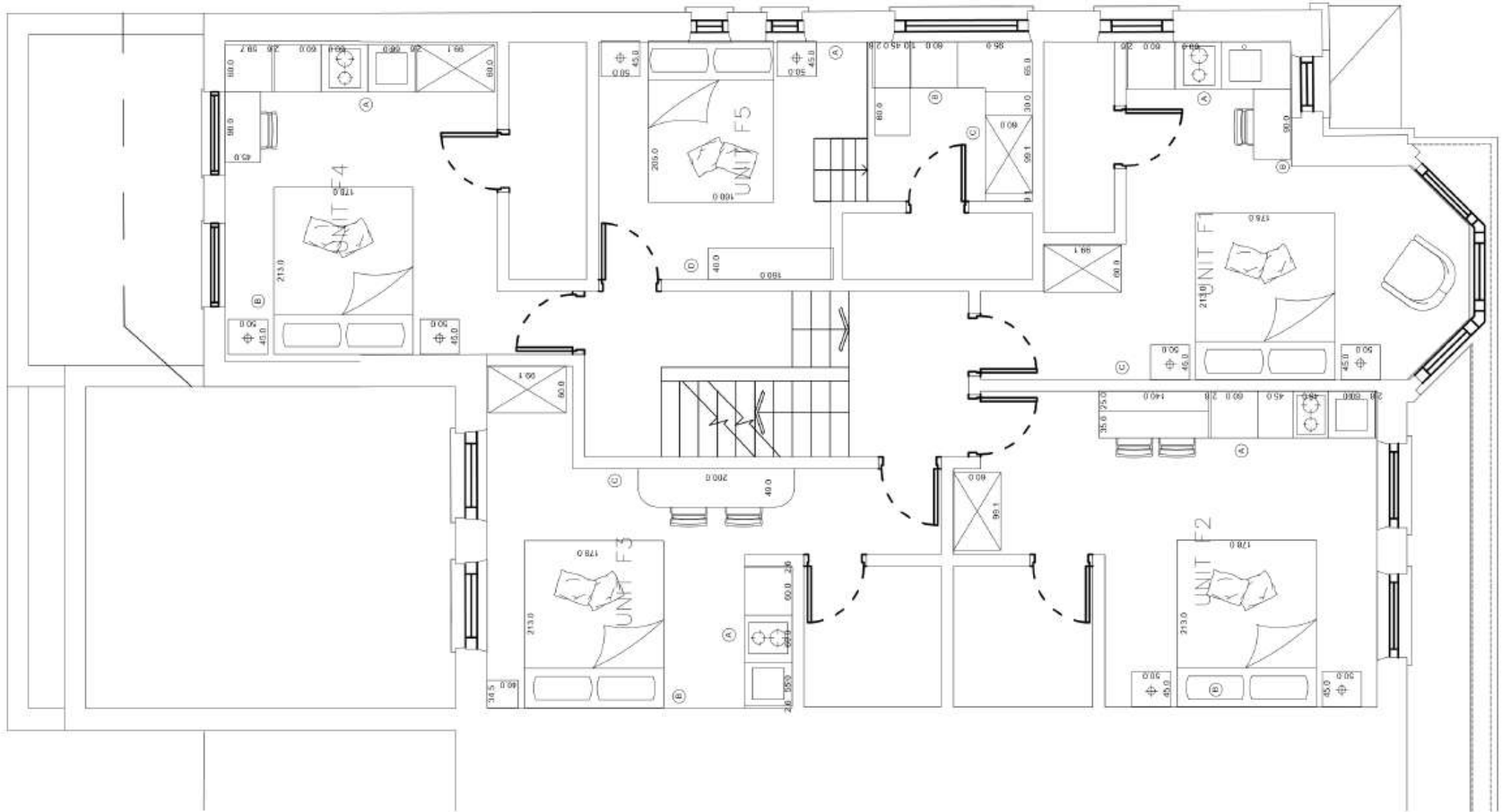
Ground Floor
