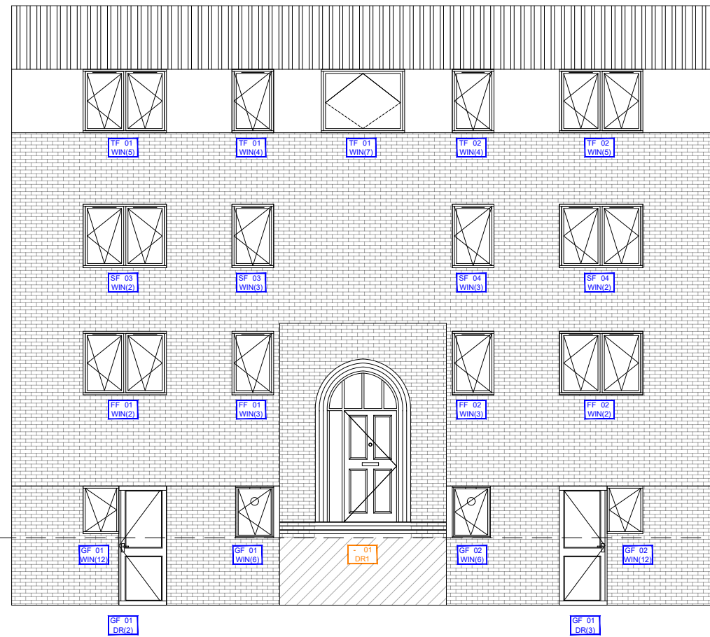
PROPOSED FRONT ELEVATION: 1:100
