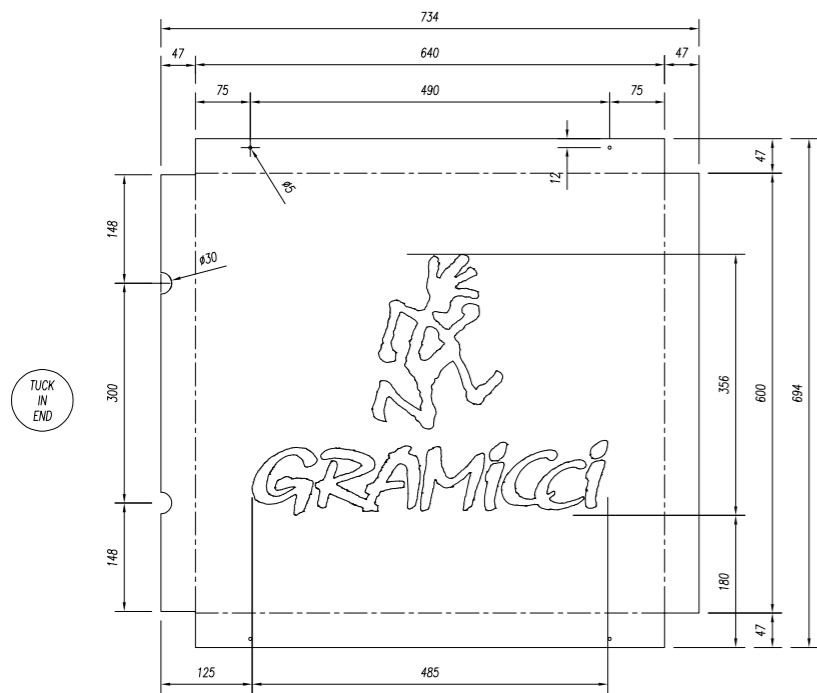
1 OFF 2mm ALUMINIUM PANEL
