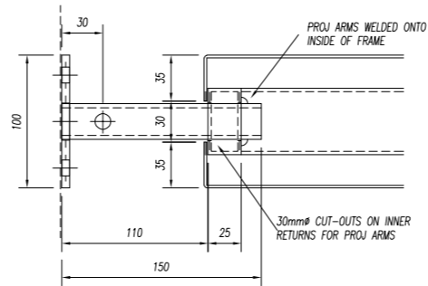
FIXING PLATE DETAIL - PLAN
