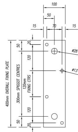
1 OFF 6MM MILD STEEL PLATE
