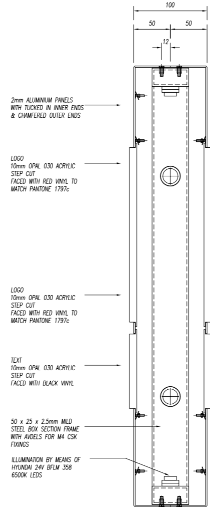
SECTION
