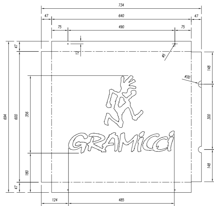
1 OFF 2mm ALUMINIUM PANEL
