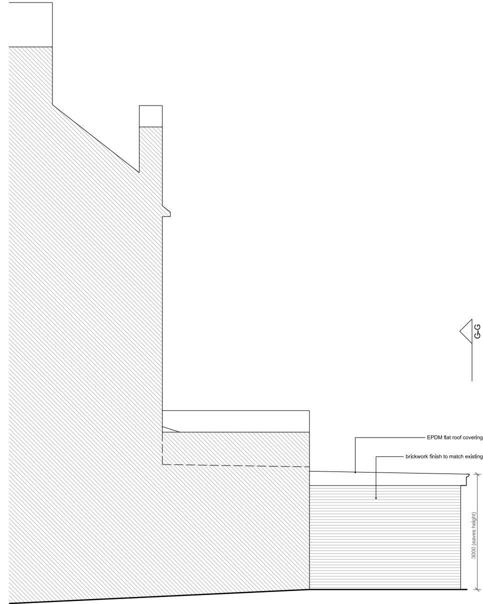
2. PROPOSED SIDE ELEVATION H-H
