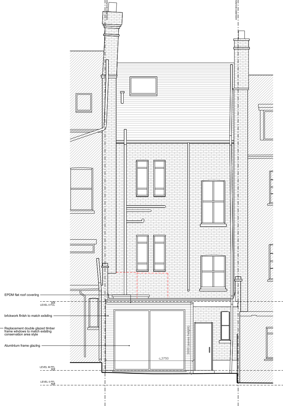
2. PROPOSED REAR ELEVATION G-G
