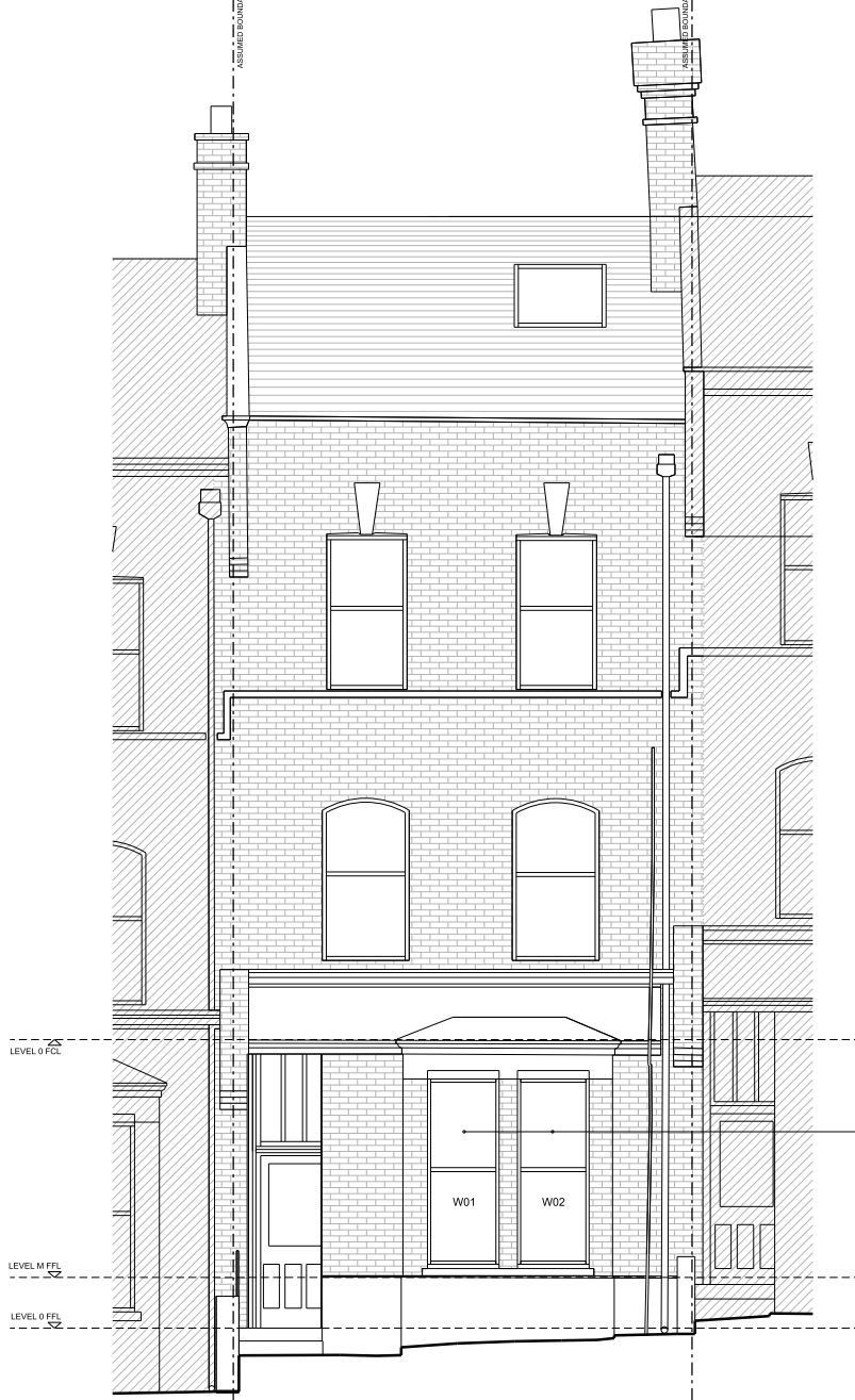
1. PROPOSED FRONT ELEVATION E-E
