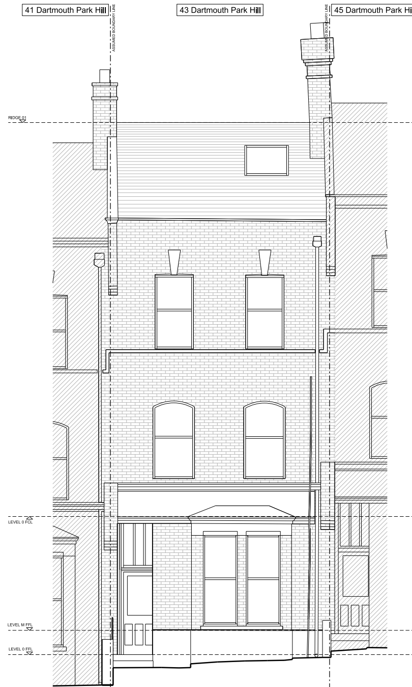
1. EXISTING FRONT ELEVATION A-A
