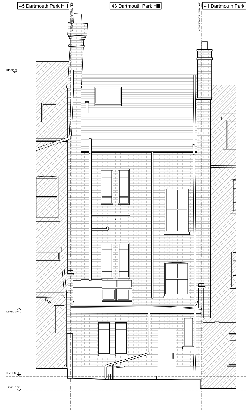
2. EXISTING REAR ELEVATION C-C
