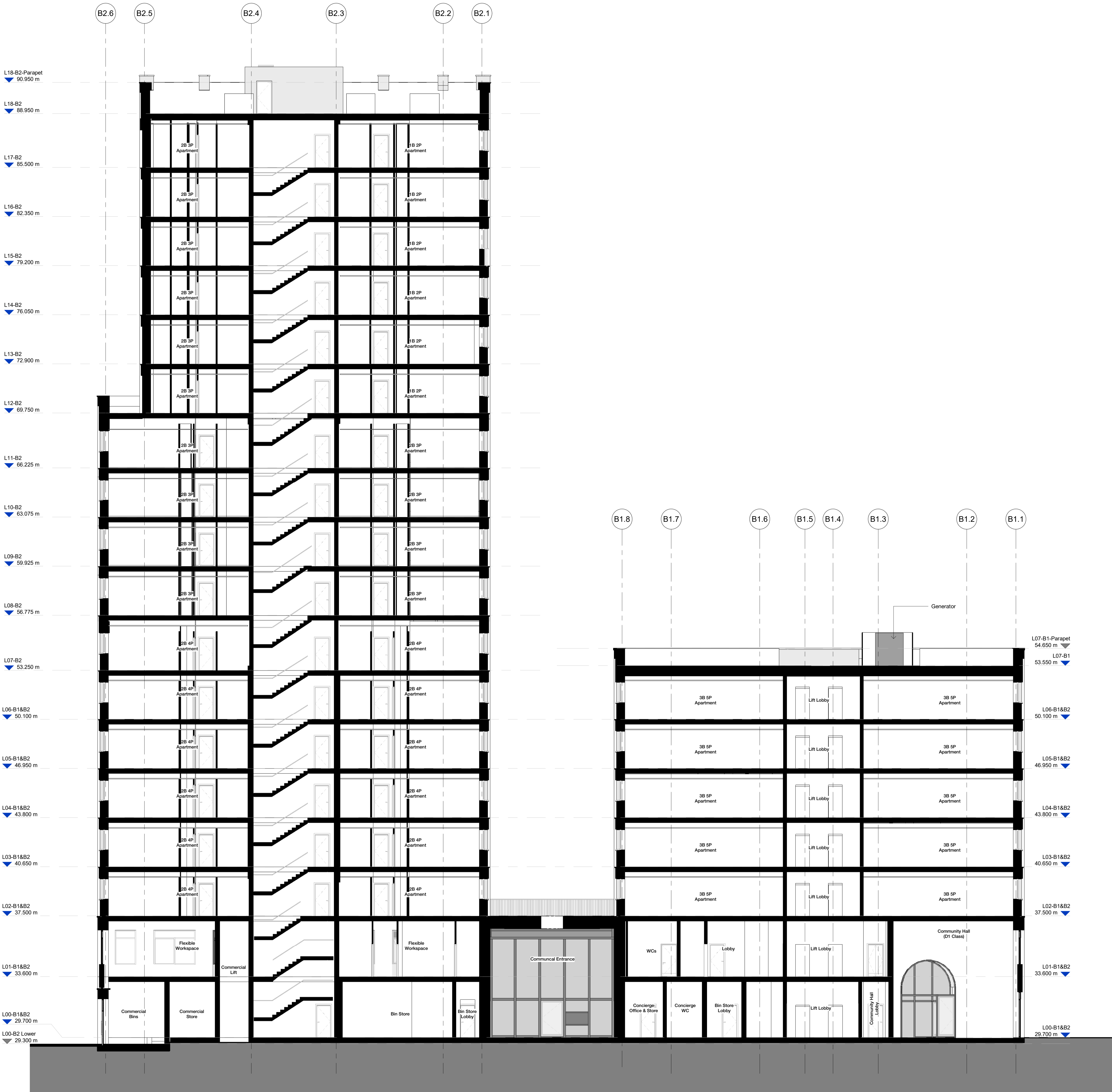
2 Long Section through B1 and B2
