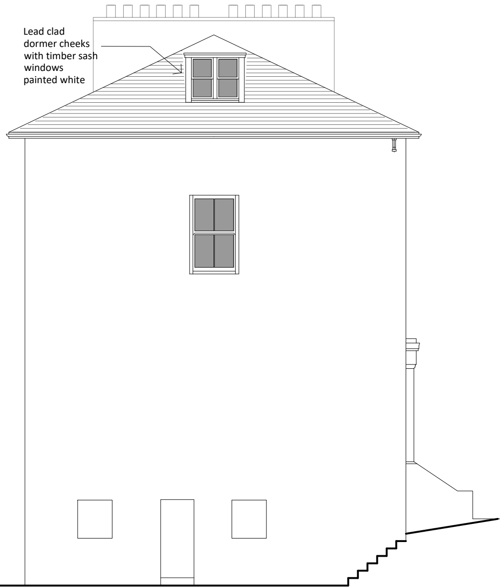
SIDE ELEVATION - PROPOSED
