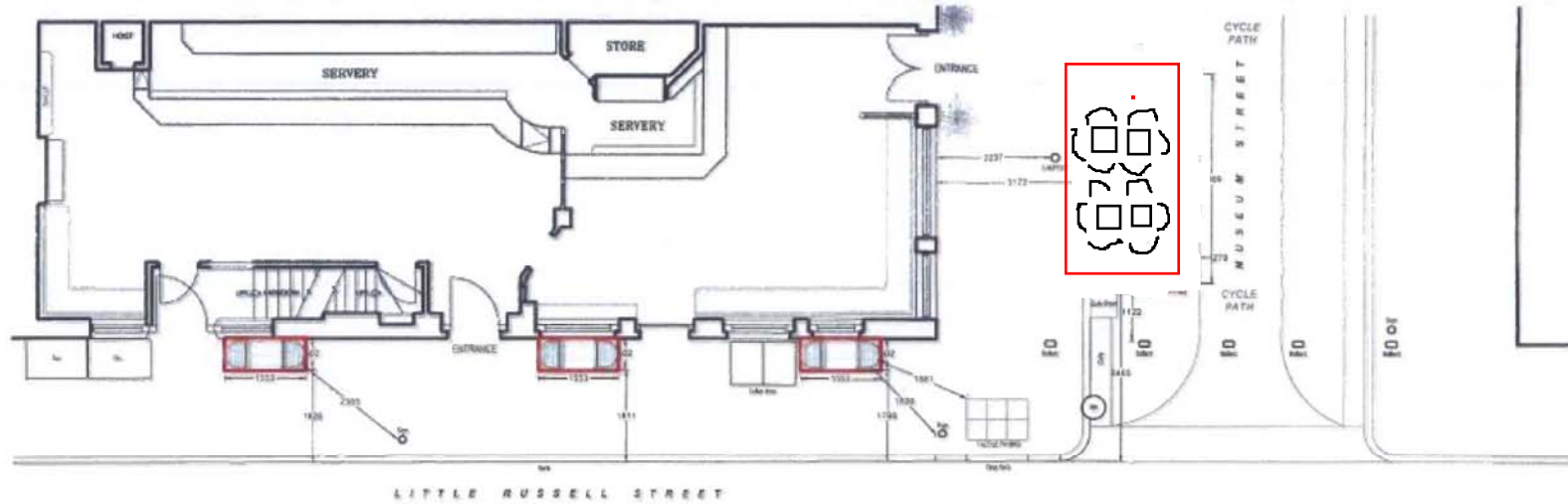
LAYOUT PLAN ( scale 1:100 )
