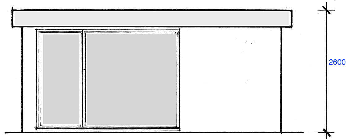
FRONT (EAST) ELEVATION
