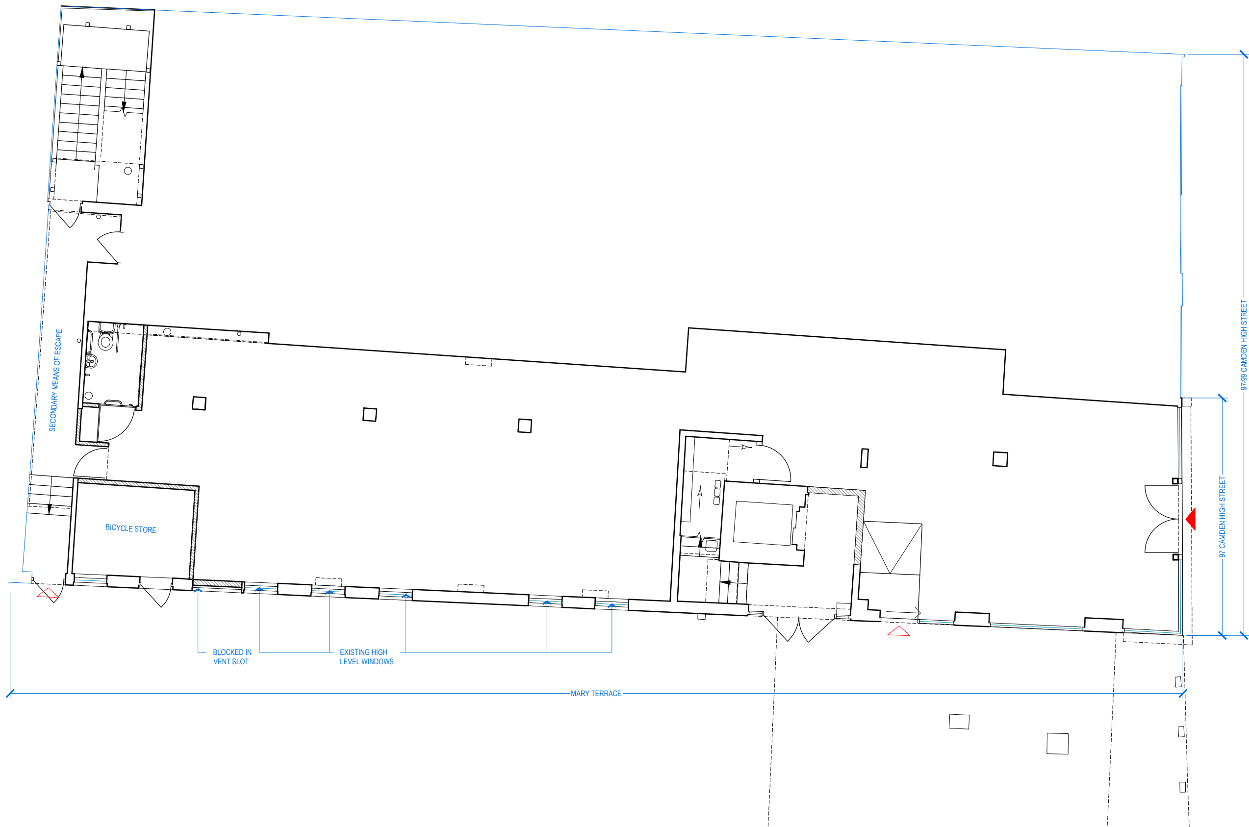
[01] EXISTING GROUND FLOOR PLAN
