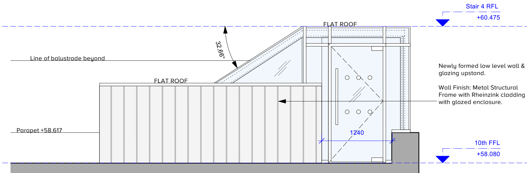
Elevation 4 (West Elevation Extract)
