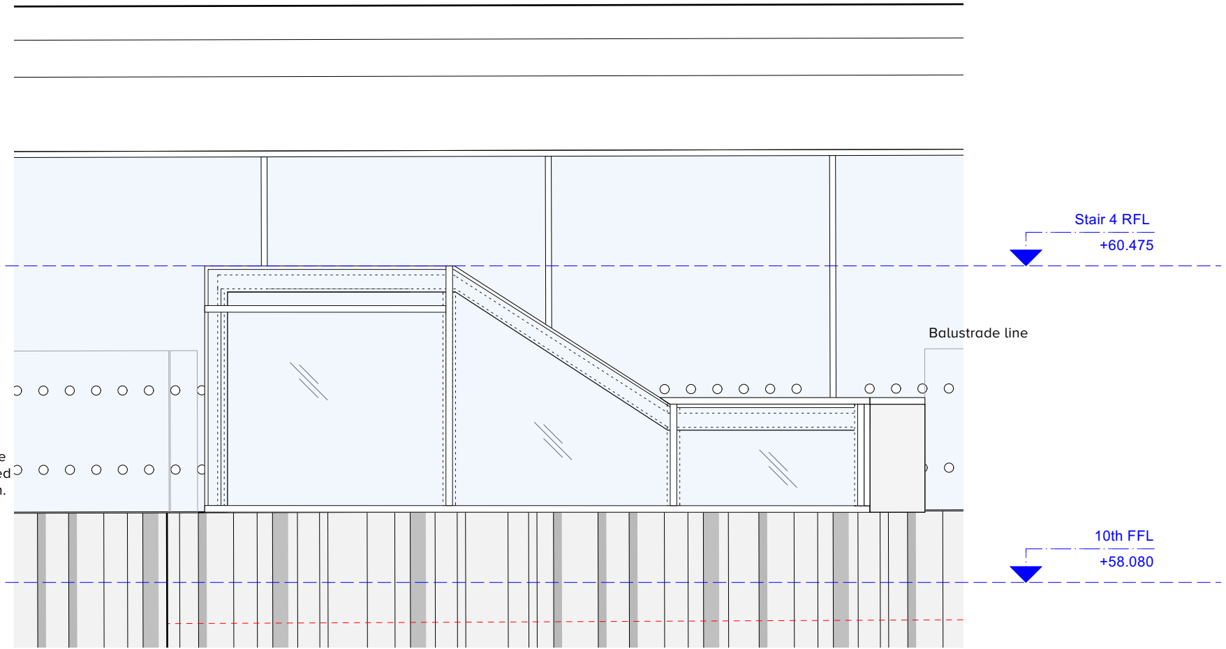
Elevation 4 (West Elevation Extract)
