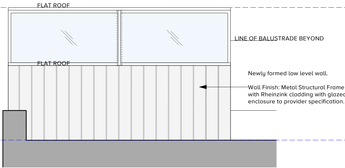
Elevation 3 - SOUTH ELEVATION
