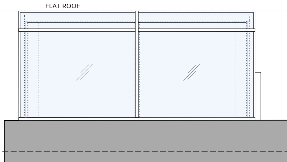
Elevation 1 - NORTH ELEVATION
