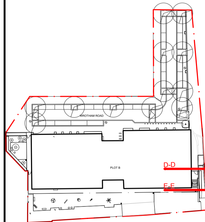
Location Plan
