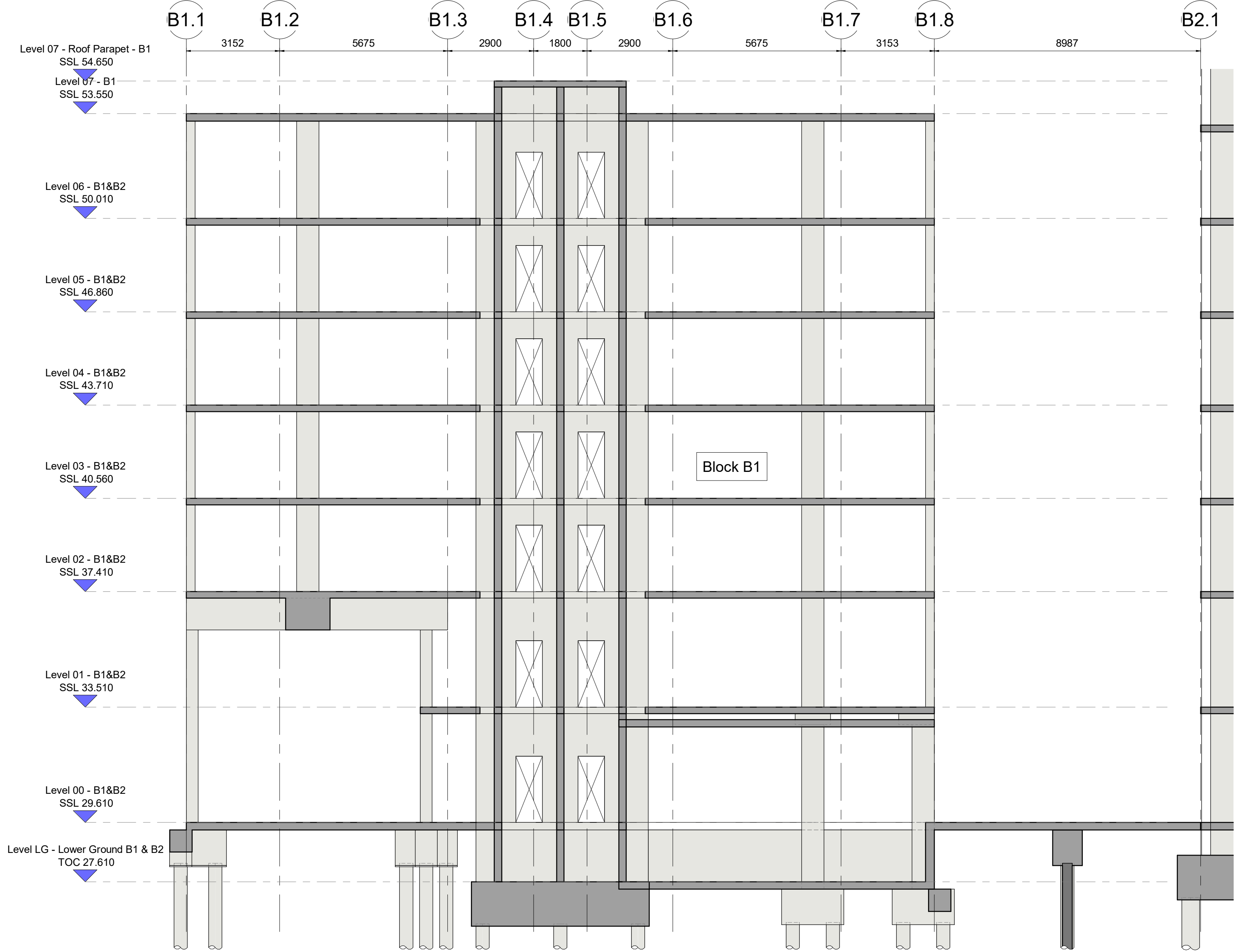
Block B1 - Long Section 2-2
