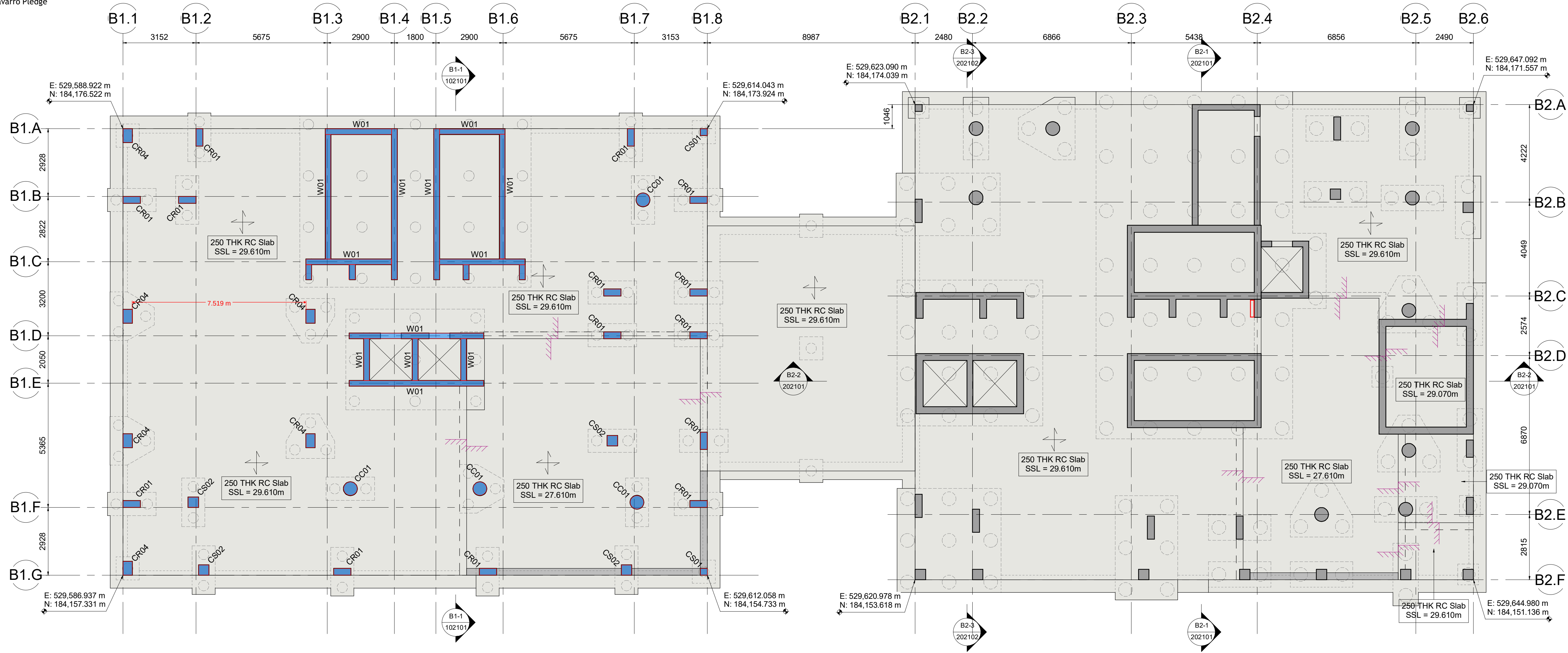
00 - Ground Floor - Block B1 & B2 1 : 100
