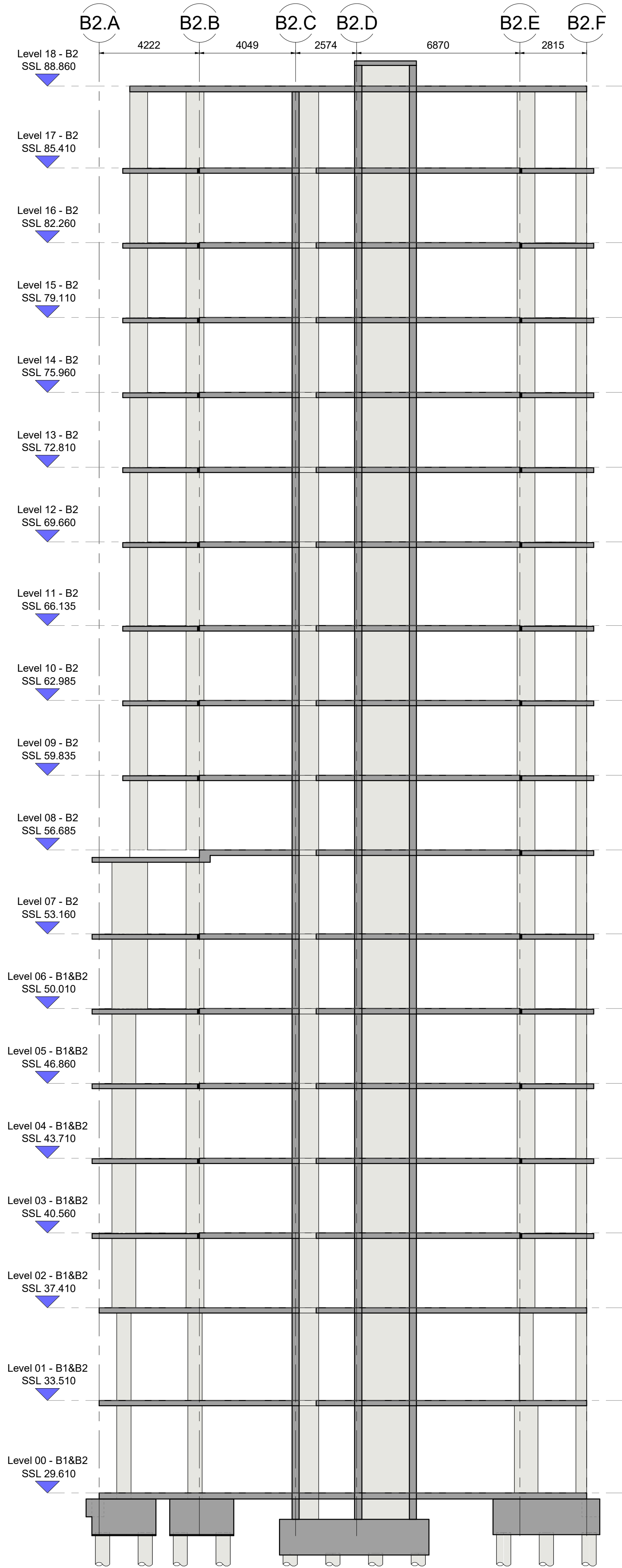
Block B2 - Long Section B2-3
