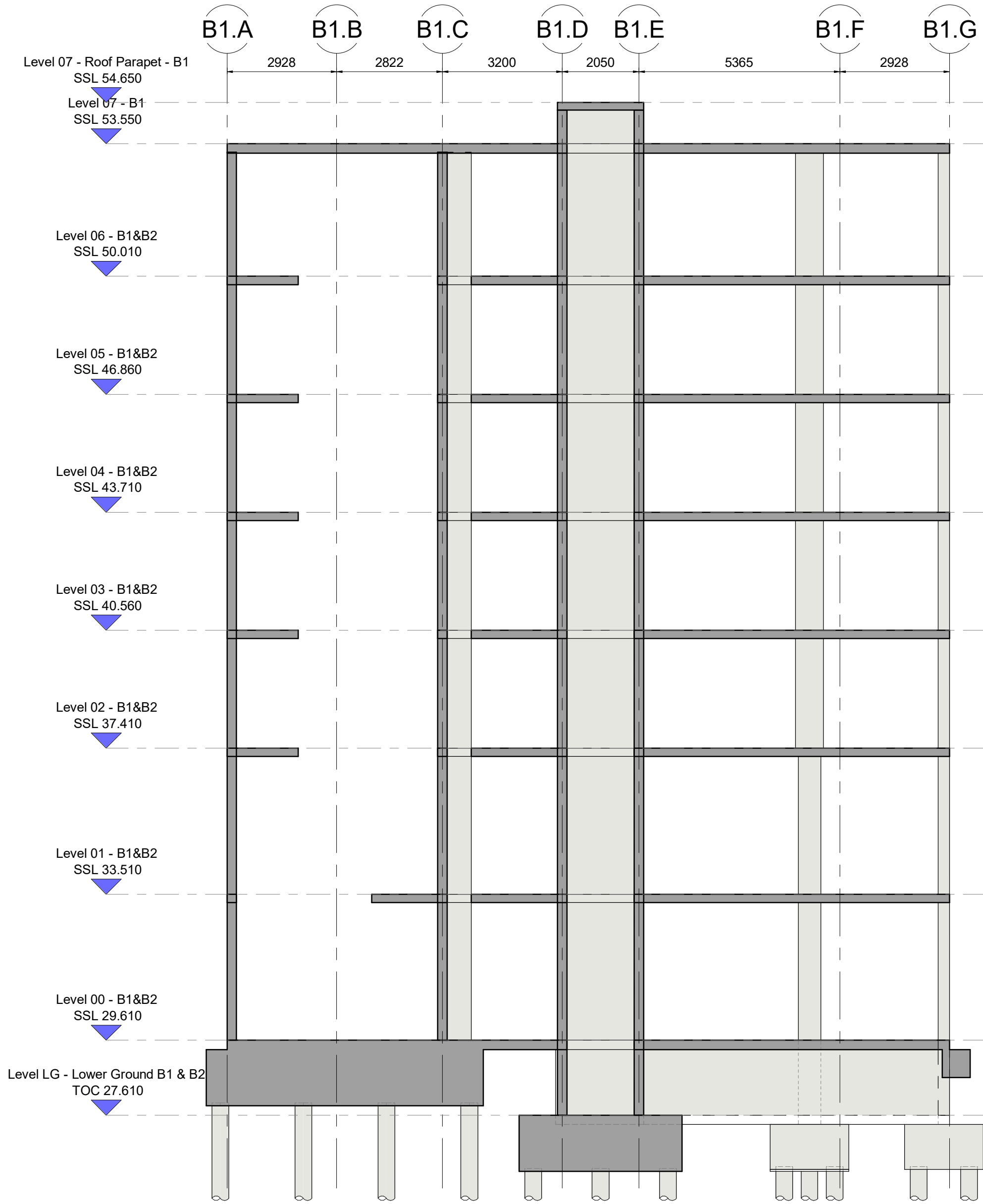
Block B1 - Long Section 1-1
