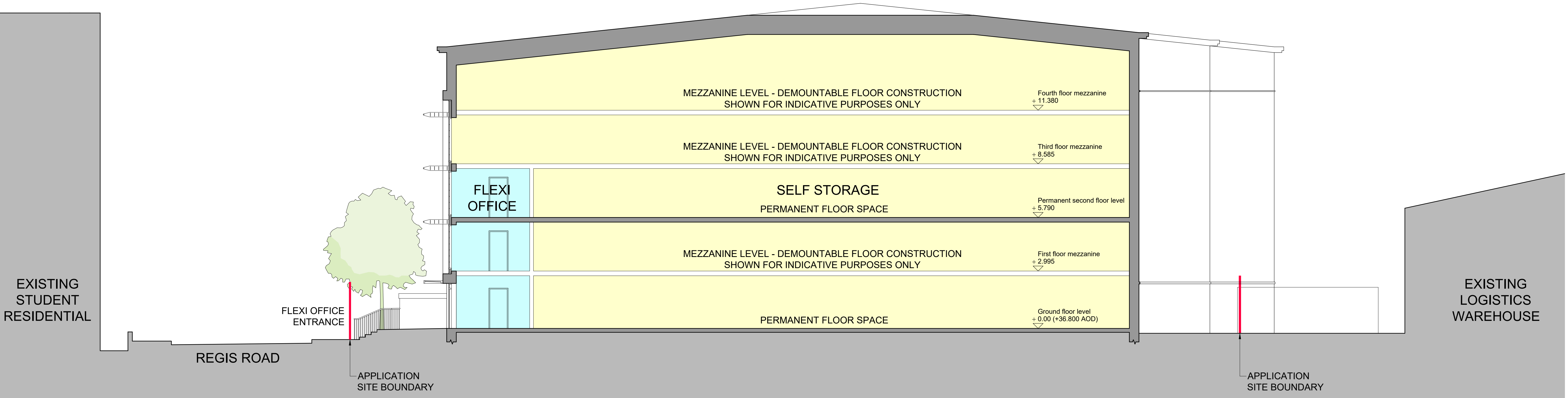
SECTION AA
