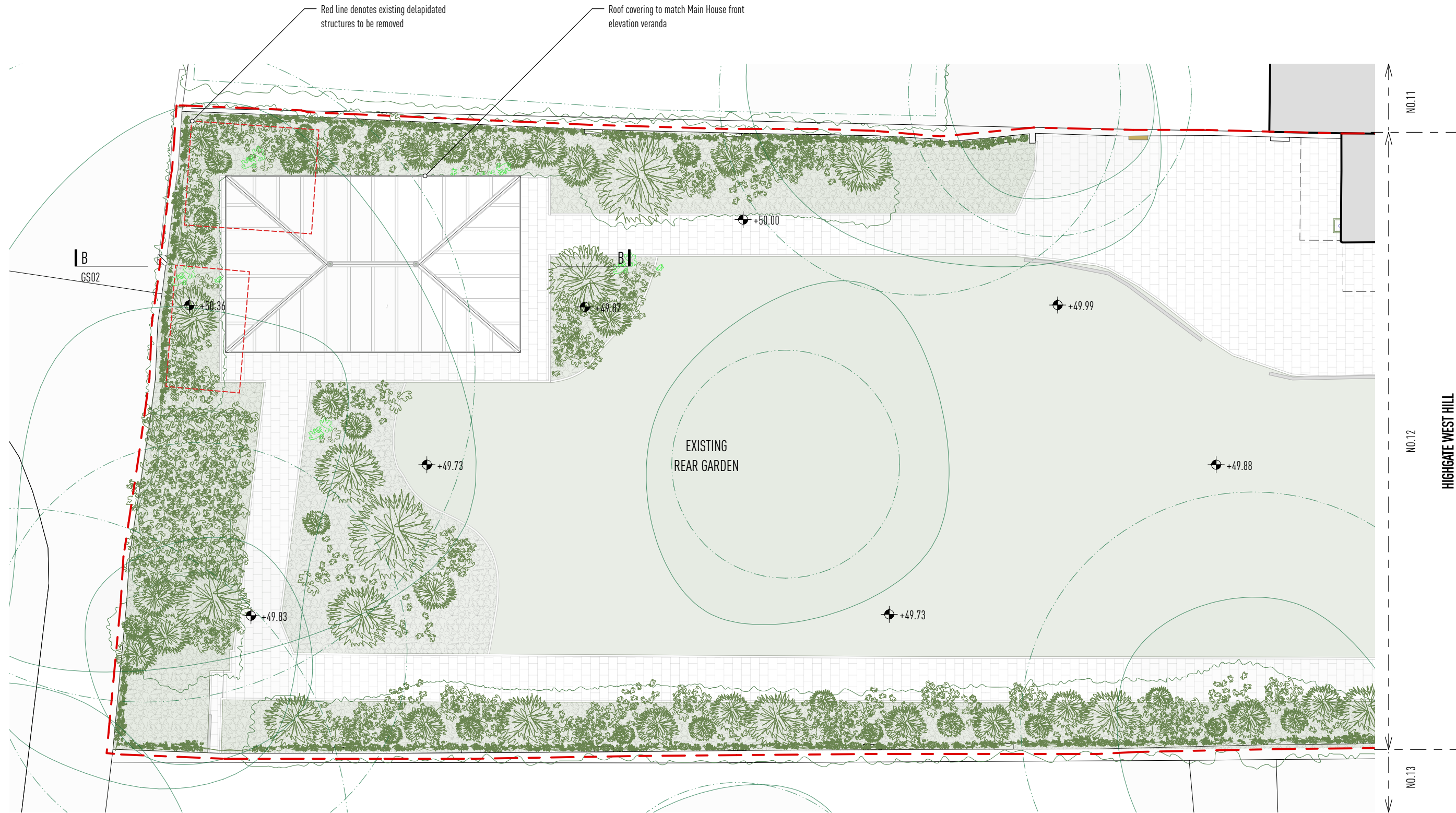
01 - Proposed Roof Plan - Summerhouse Scale 1:100@A3
